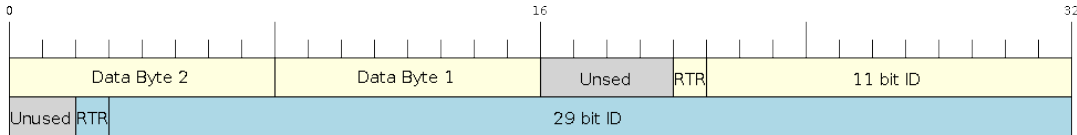
Fig. 14: Bit layout of single filter mode (Right side MSBit)
