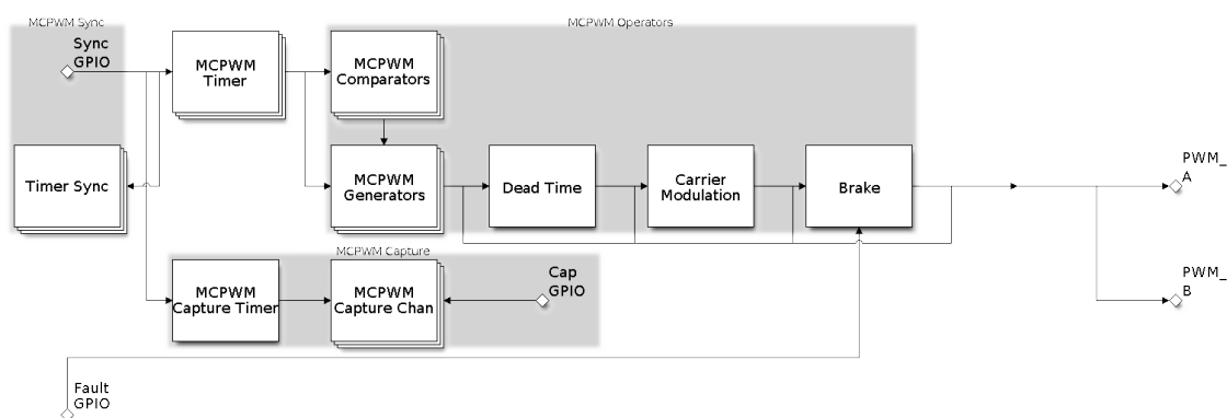
Fig. 8: MCPWM Overview
