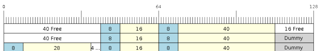
Fig. 34: Wrap around in No-Split buffers
