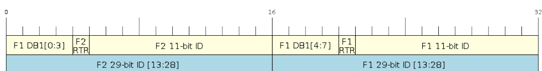
Fig. 22: Bit layout of dual filter mode (Right side MSBit)
