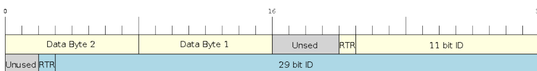
Fig. 25: Bit layout of single filter mode (Right side MSBit)
