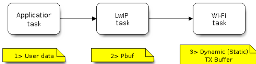
Fig. 62: TX Buffer Allocation
