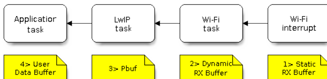
Fig. 35: RX Buffer Allocation
