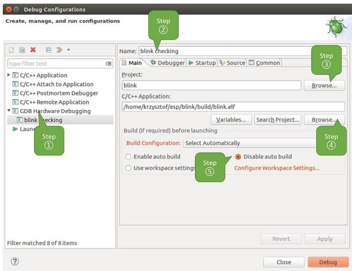
Fig. 58: Configuration of GDB Hardware Debugging - Main tab
