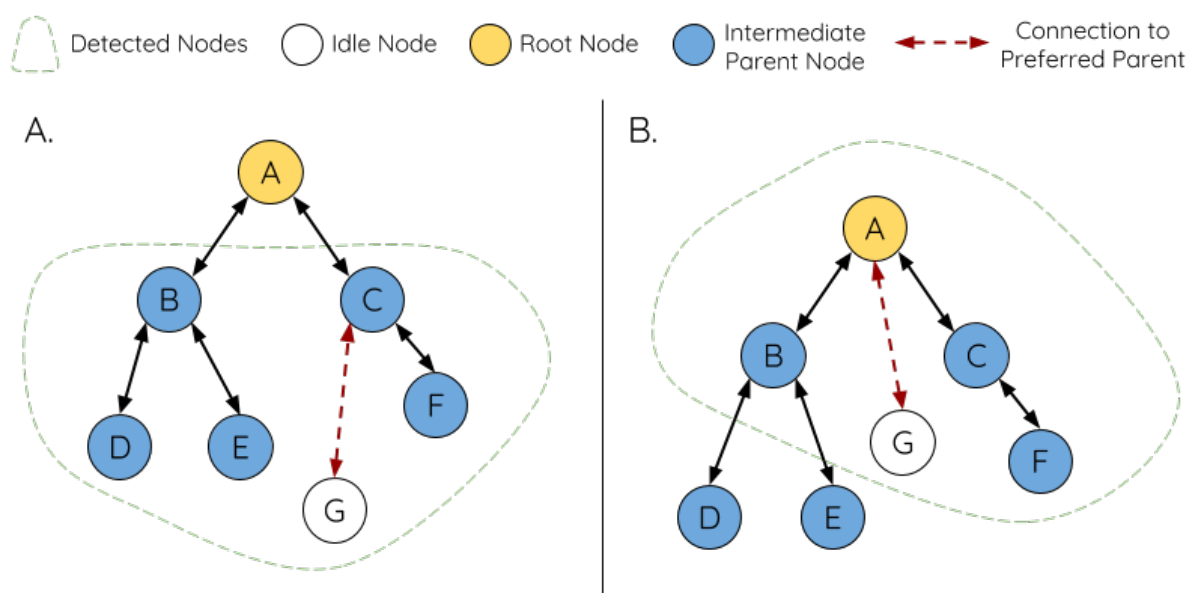
Fig. 45: Preferred Parent Node Selection
