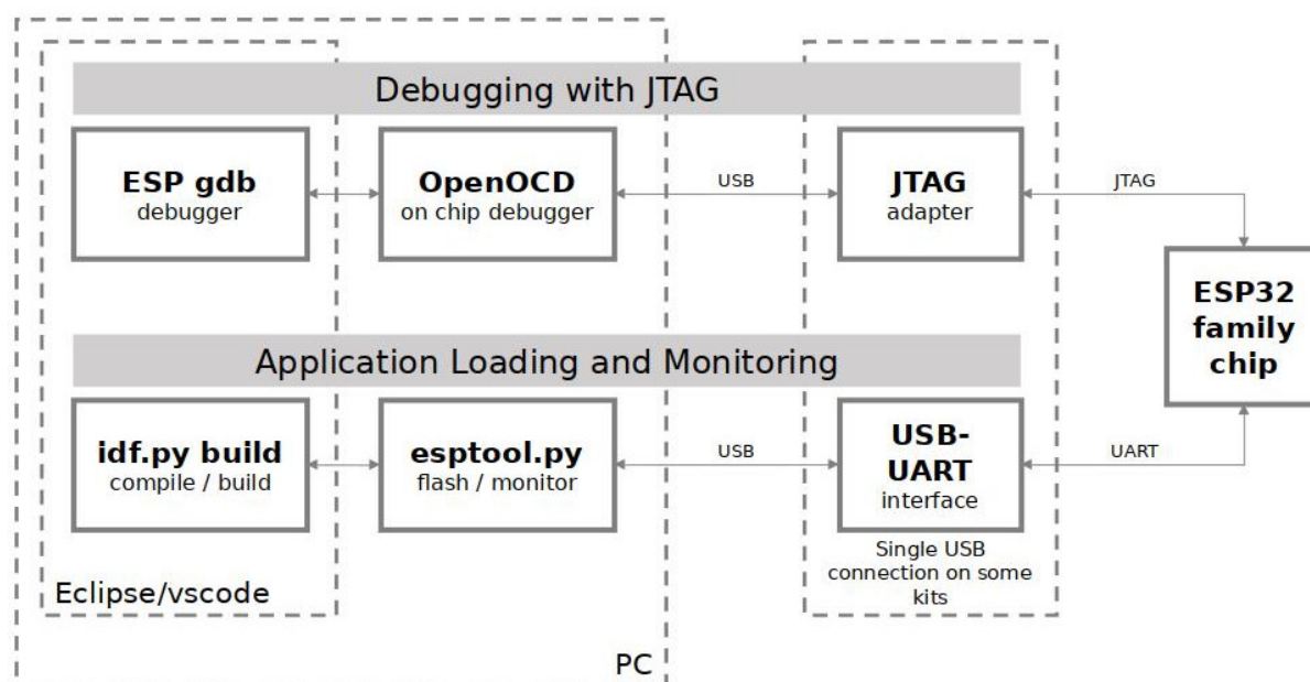
Fig. 57: JTAG debugging - overview diagram
