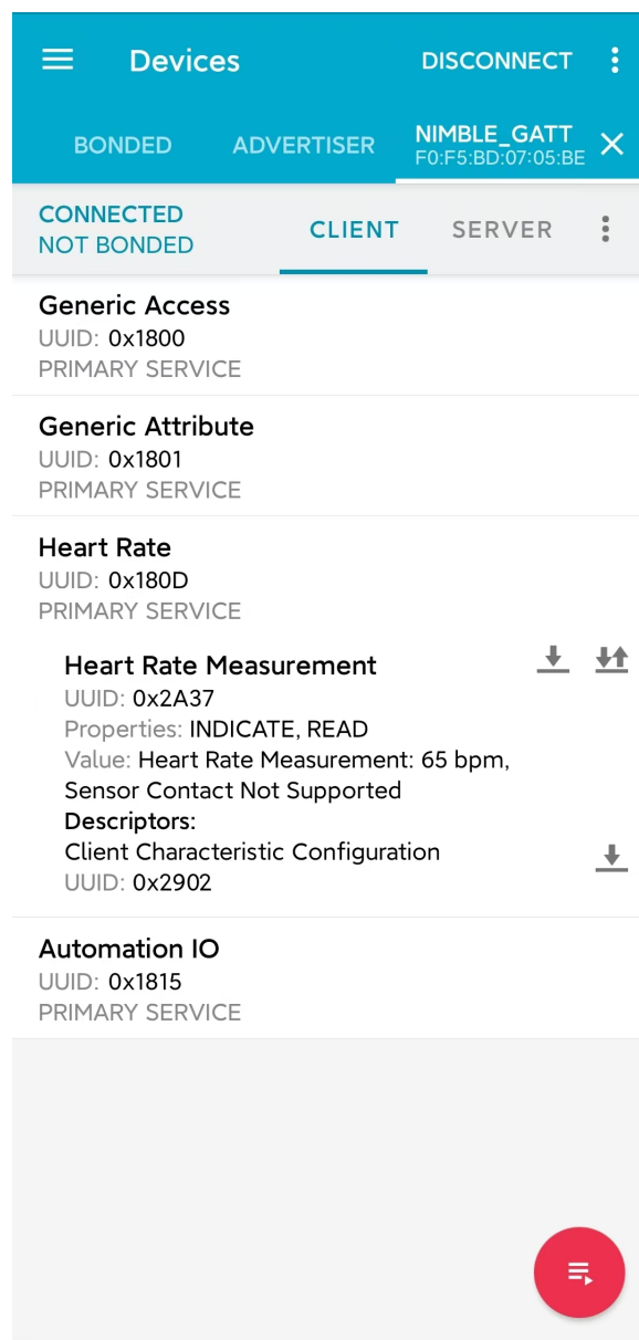
Fig. 12: Read Heart Rate Characteristic Data
