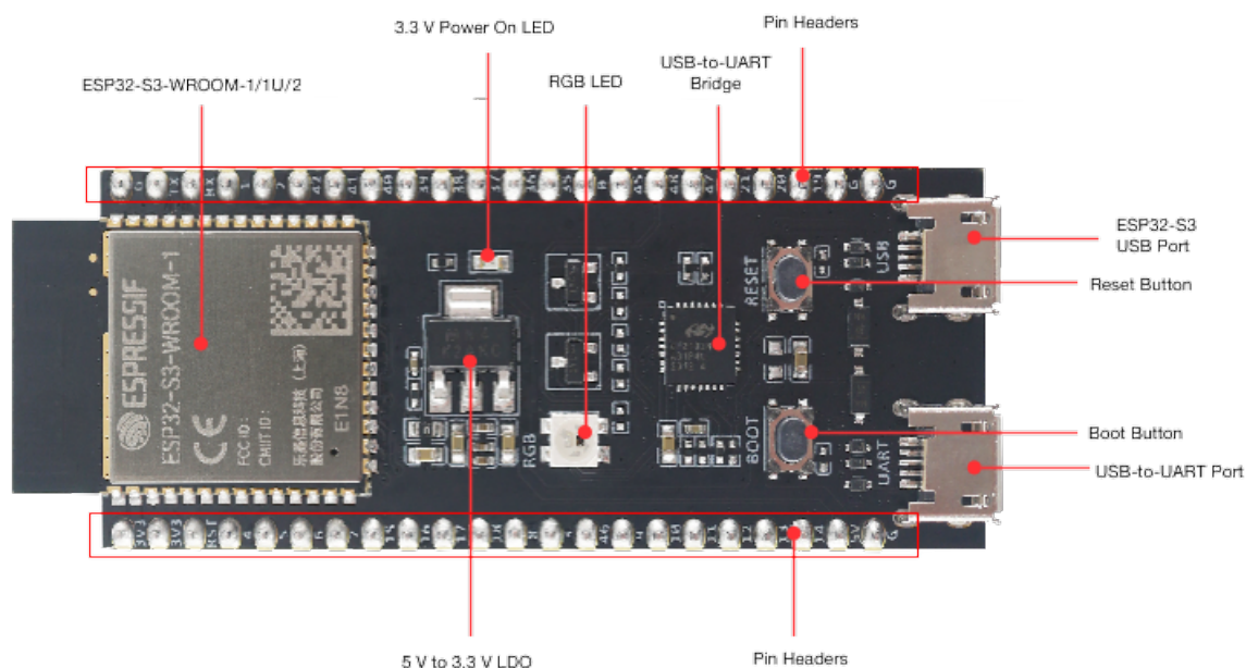
Fig. 2: ESP32-S3-DevKitC-1 - front
