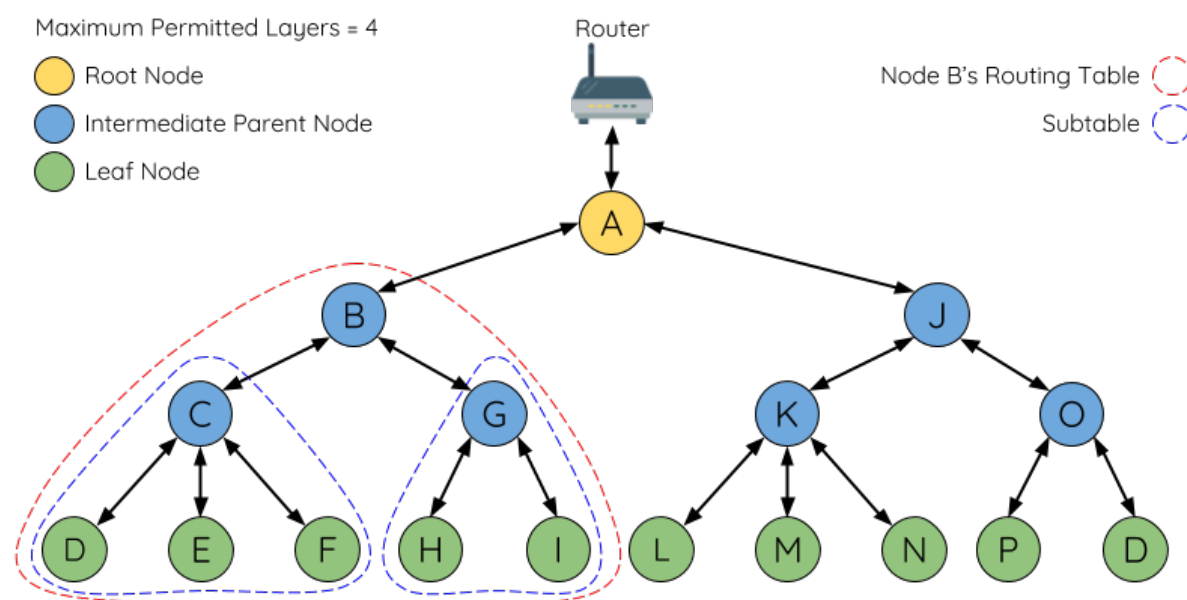
Fig. 46: ESP-WIFI-MESH Routing Tables Example
