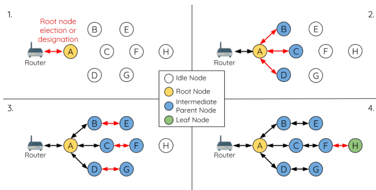
Fig. 47: ESP-WIFI-MESH Network Building Process
