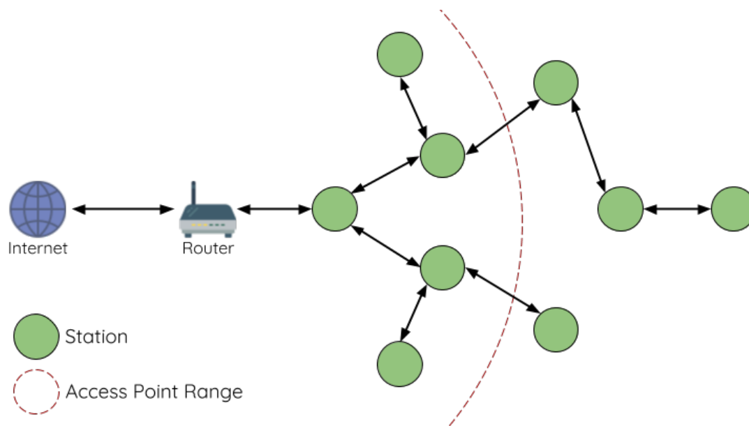
Fig. 41: ESP-WIFI-MESH Network Architecture
