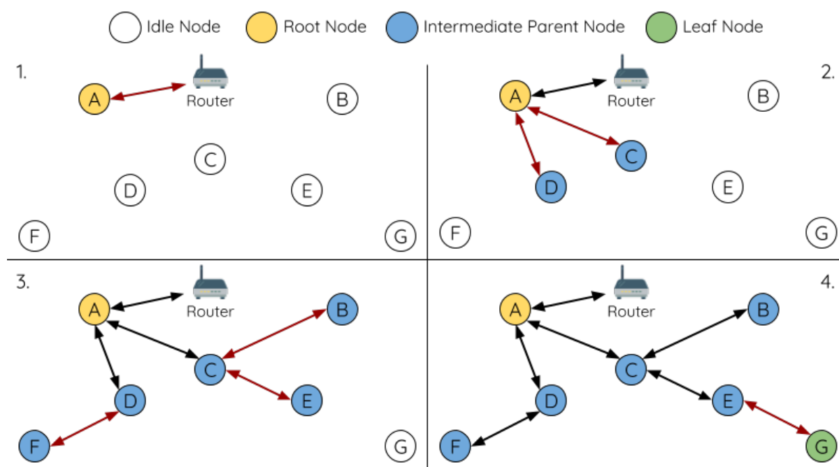
Fig. 49: Root Node Designation Example (Root Node = A, Max Layers = 4)
