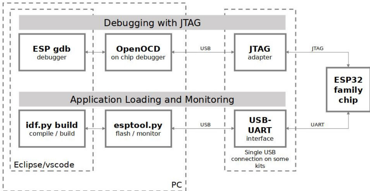
Fig. 8: JTAG debugging - overview diagram
