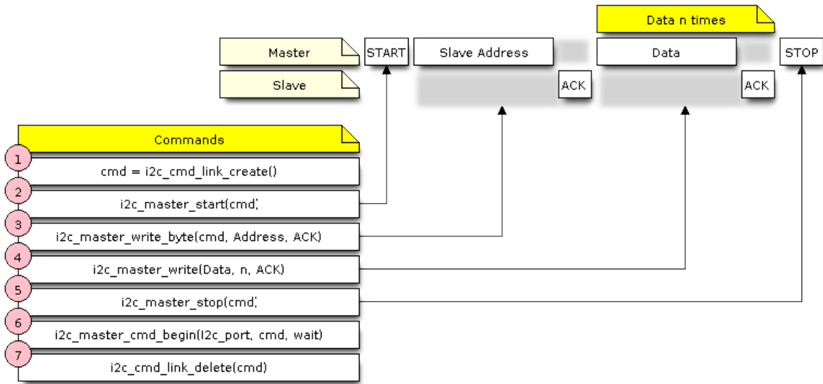
Fig. 6: I2C command link - master write example
