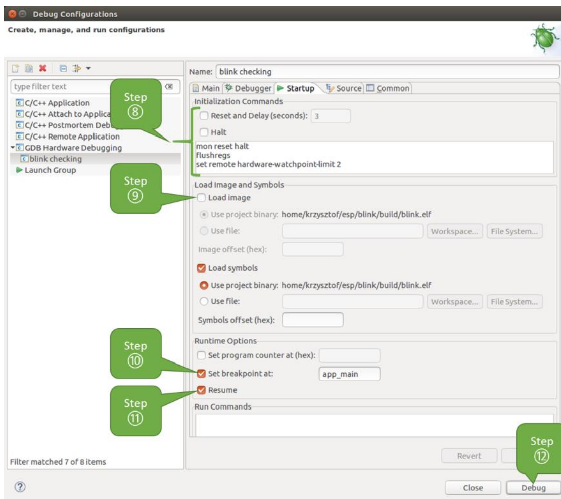
Fig. 22: Configuration of GDB Hardware Debugging - Startup tab
