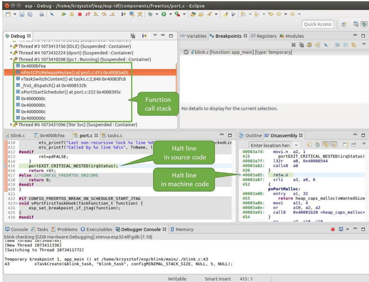
Fig. 26: Navigate through the call stack
