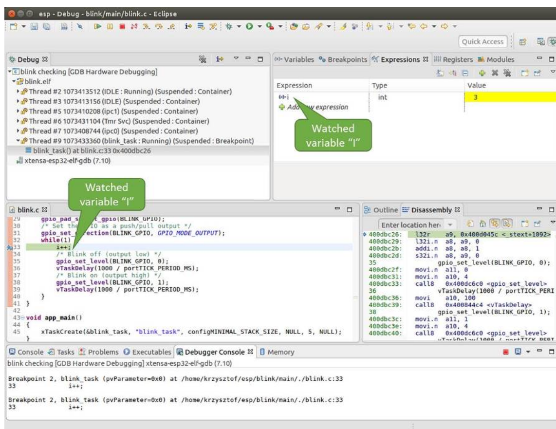
Fig. 34: Watching program variable “i”
