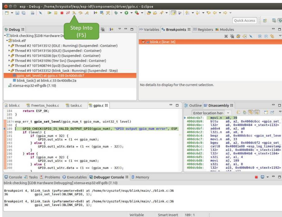
Fig. 31: Stepping through the code with “Step Into (F5)”
