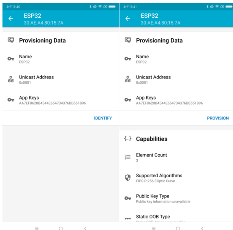
Fig. 10: nRF Mesh - IDENTIFY - PROVISION
