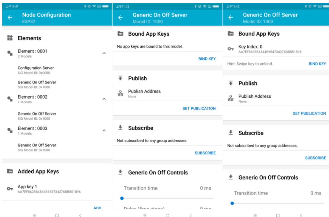
Fig. 15: nRF Mesh - Model Bind AppKey
