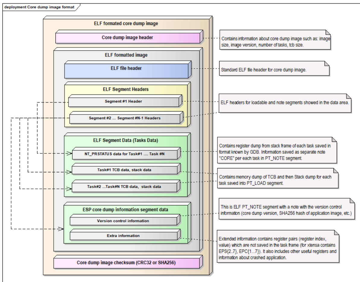
Fig. 5: Core Dump ELF Image Format
