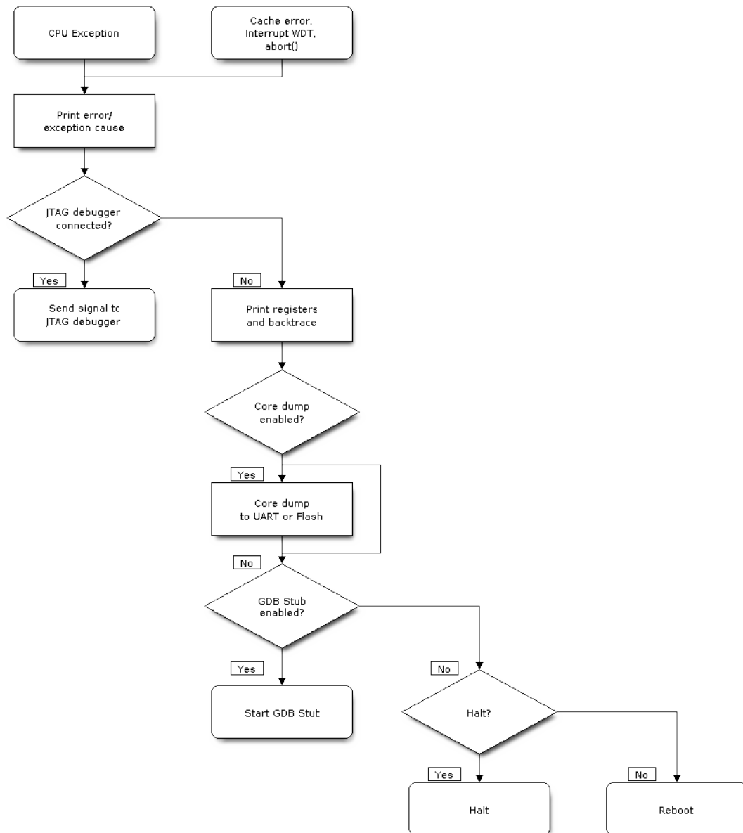
Fig. 20: Panic Handler Flowchart (click to enlarge)
