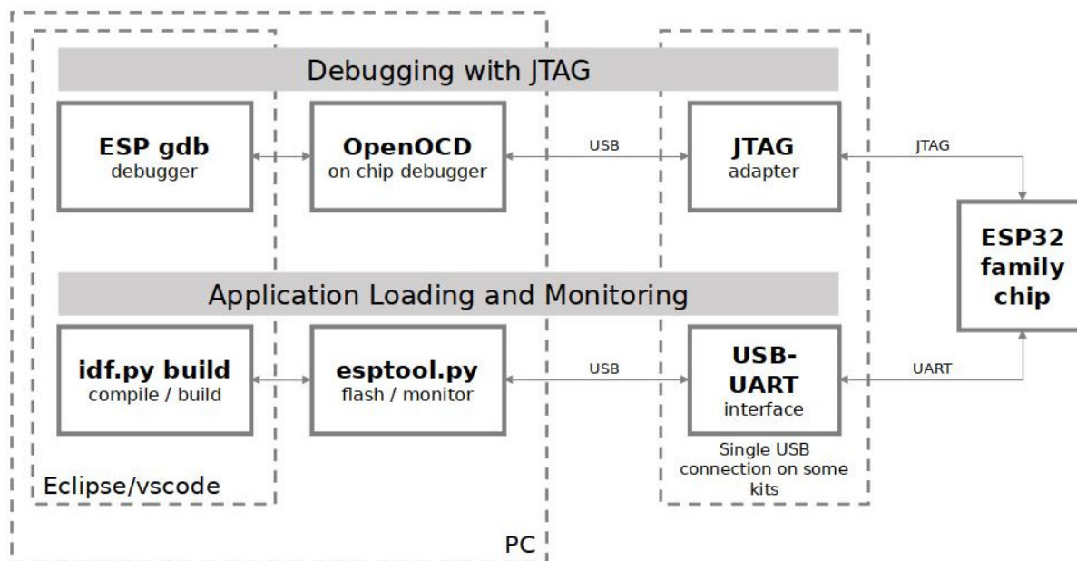
Fig. 21: JTAG debugging - overview diagram
