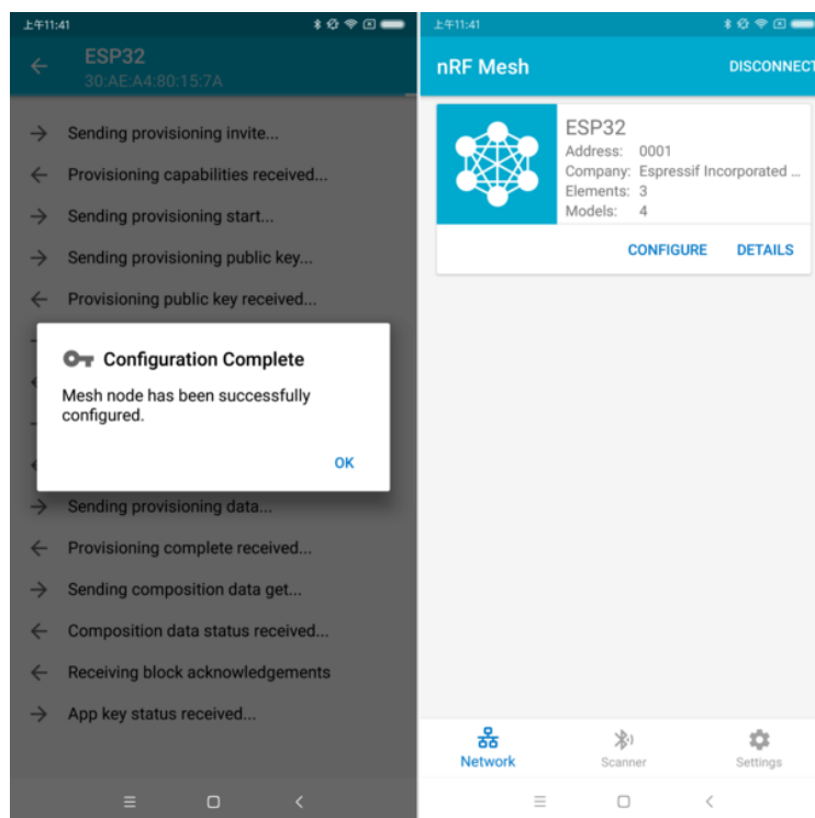
Fig. 11: nRF Mesh - Configuration Complete
