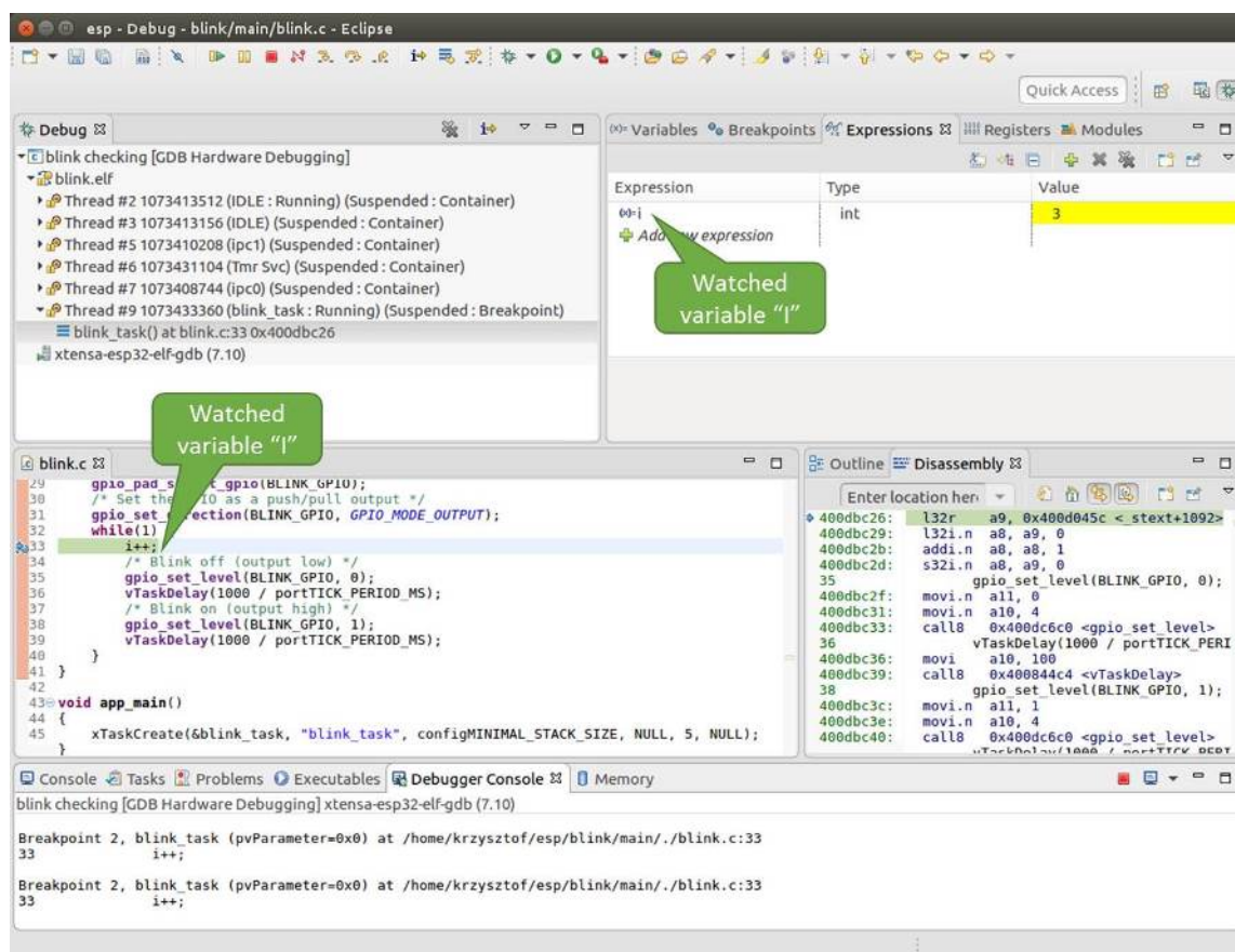
Fig. 56: Watching program variable "i"
