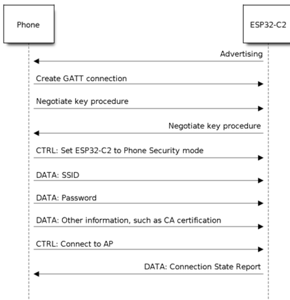
Fig. 3: BluFi Flow Chart
