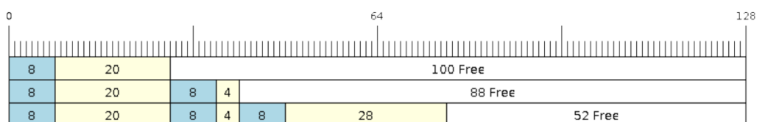
Fig. 10: Sending items to No-Split or Allow-Split ring buffers
