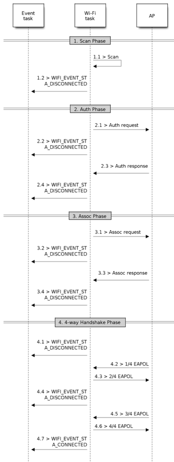
Fig. 35: Wi-Fi Station Connecting Process
