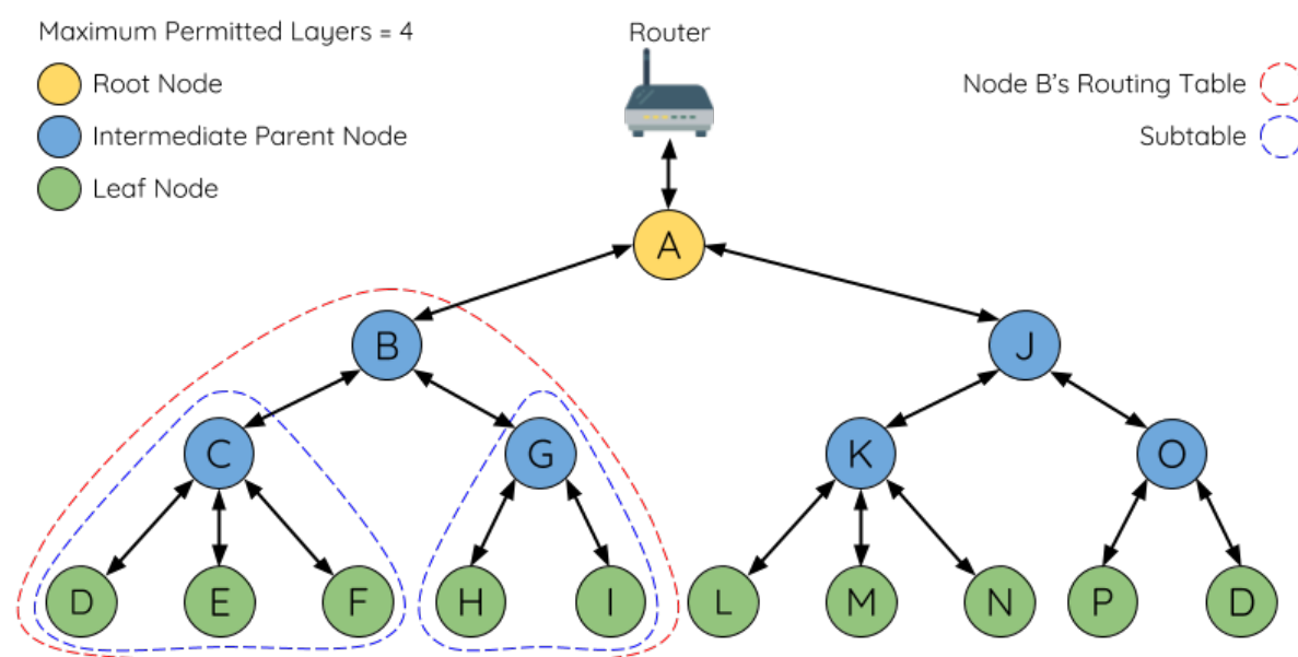
Fig. 28: ESP-WIFI-MESH Routing Tables Example
