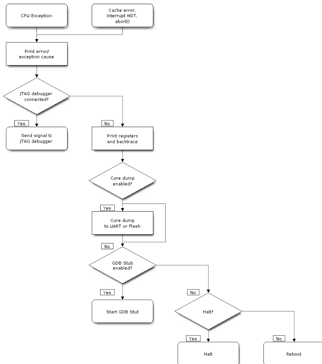
Fig. 21: Panic Handler Flowchart (click to enlarge)
