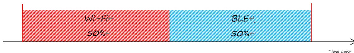
Fig. 17: Time Slice Under the Status of Wi-Fi CONNECTED and BLE CONNECTED
