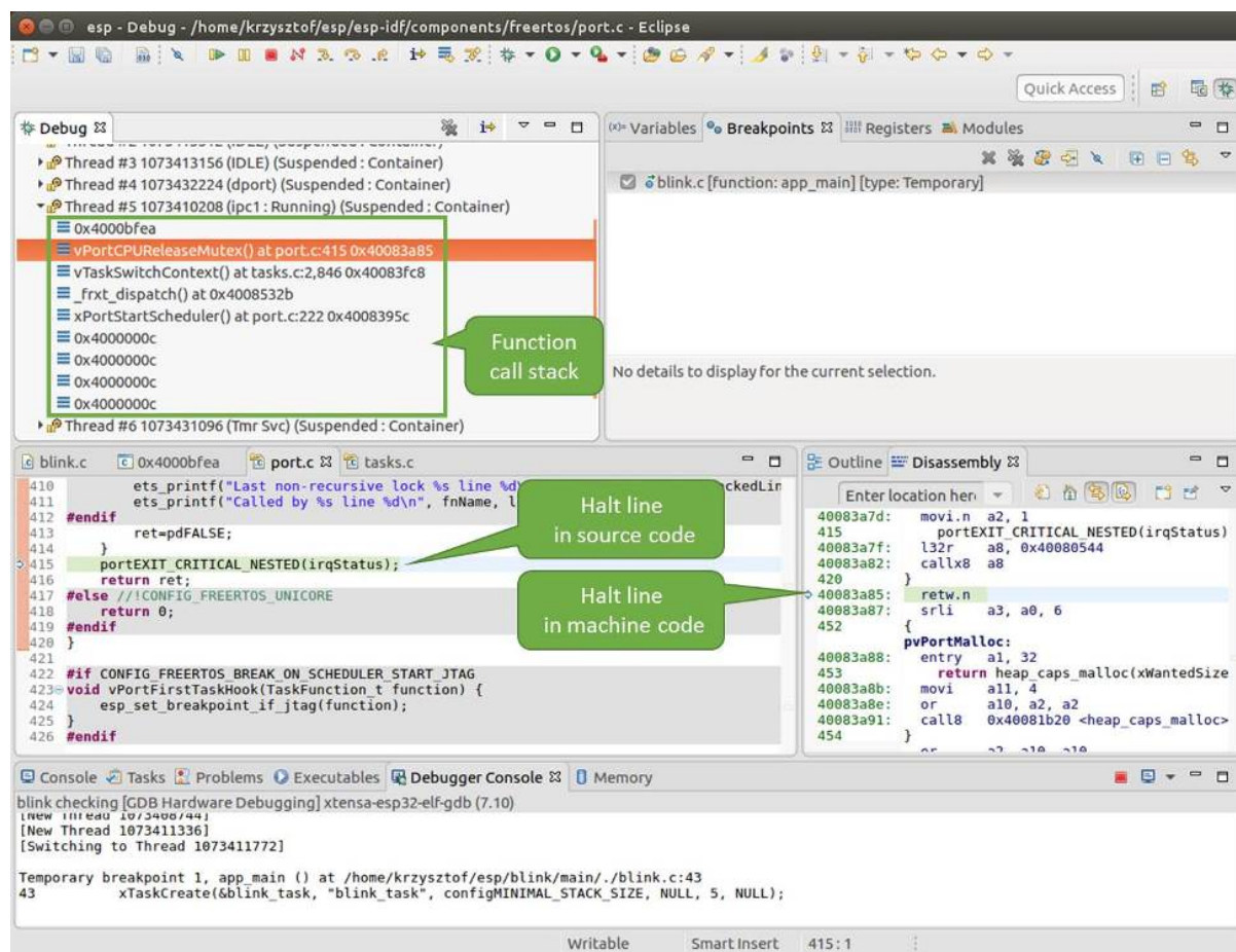
Fig. 29: Navigate through the call stack
