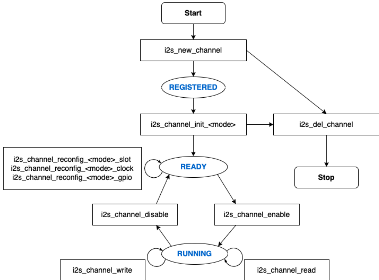
Fig. 7: I2S Finite State Machine
