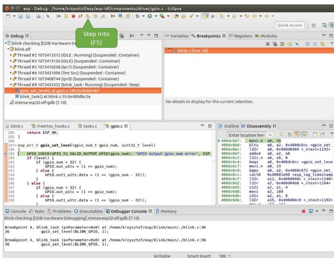
Fig. 34: Stepping through the code with "Step Into (F5)"
