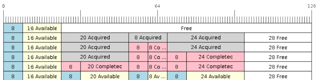
Fig. 12: SendAcquire / SendComplete items in No-Split ring buffers
