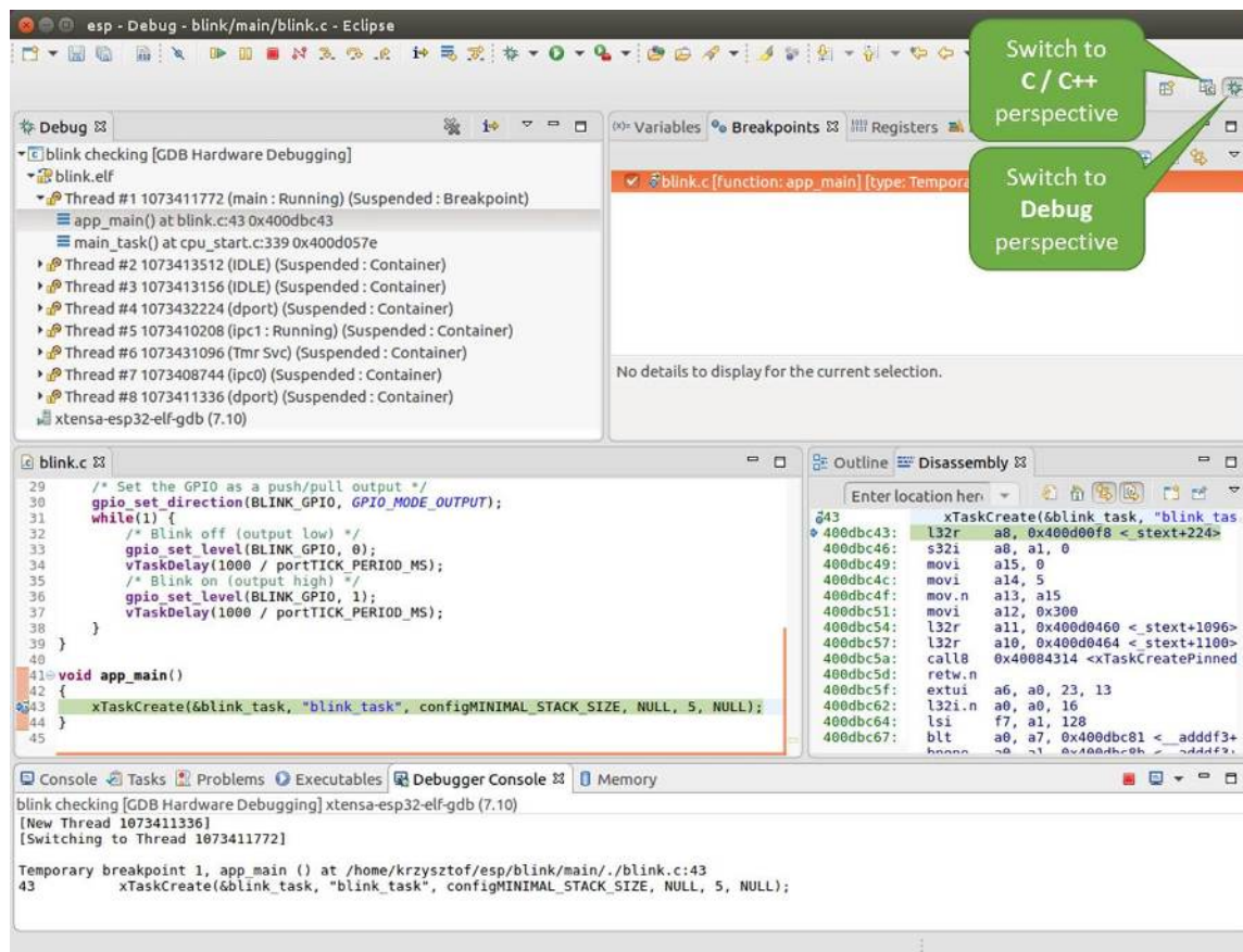
Fig. 12: Debug Perspective in Eclipse
