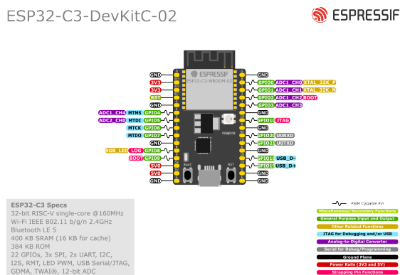
Fig. 8: ESP32-C3-DevKitC-02 Pin Layout (click to enlarge)
