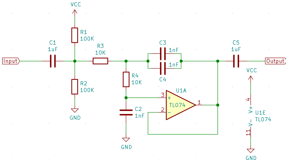
Fig. 18: Sallen-Key Low Pass Filter
