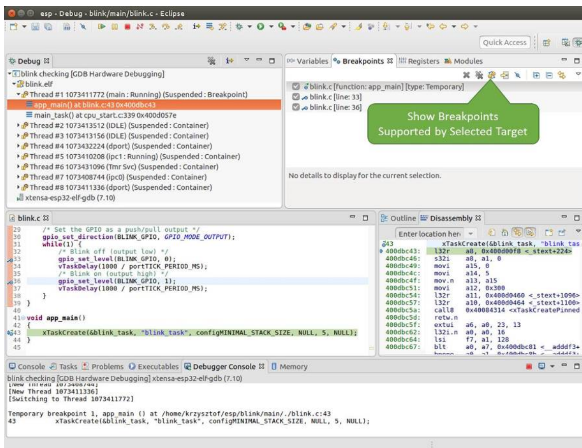
Fig. 21: Three breakpoints are set / maximum two are allowed
