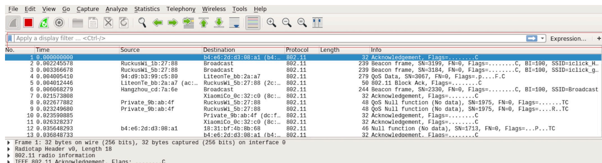
Fig. 41: Setting up Filters in Wireshark
