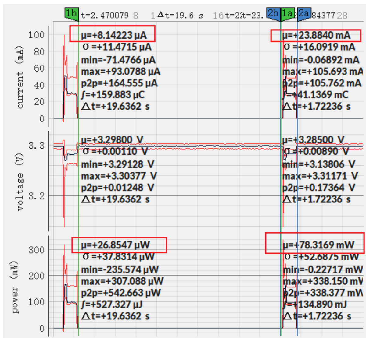
Fig. 9: Current Waveform of ESP32-S3-WROOM-1 (click to enlarge)
