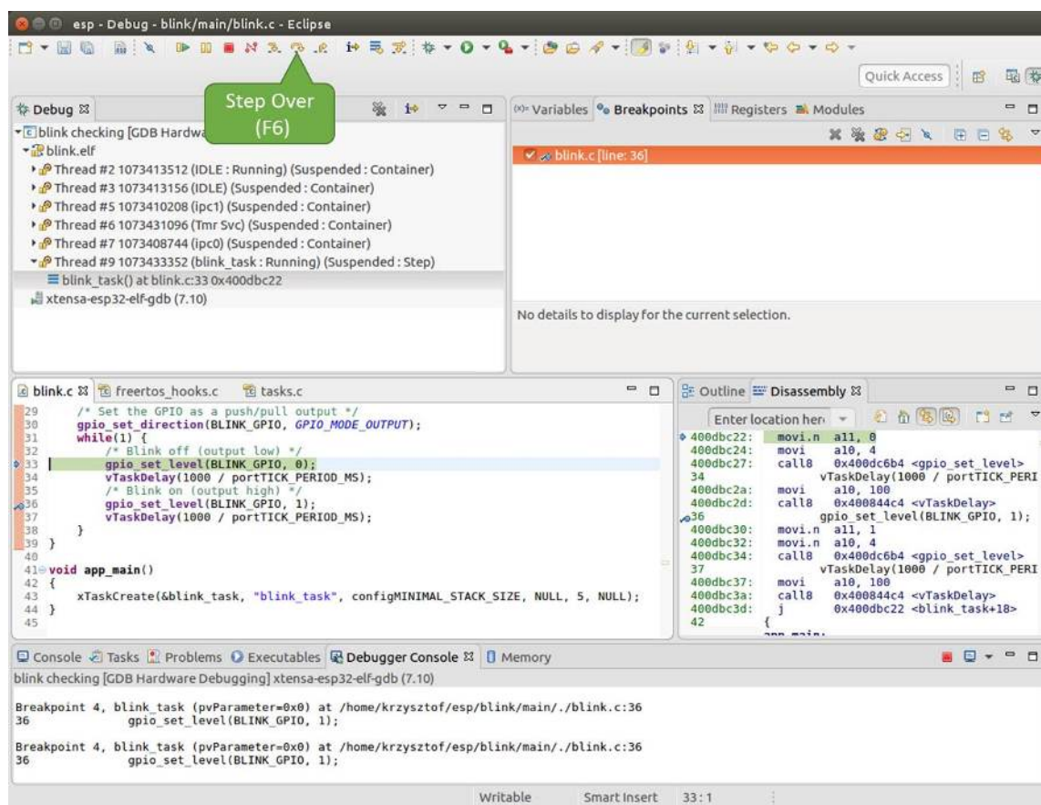
Fig. 23: Stepping through the code with "Step Over (F6)"
