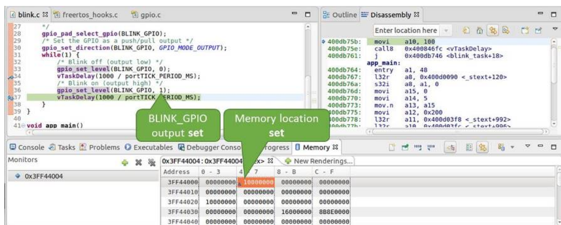
Fig. 25: Observing memory location 0x3FF44004 changing one bit to "ON"
