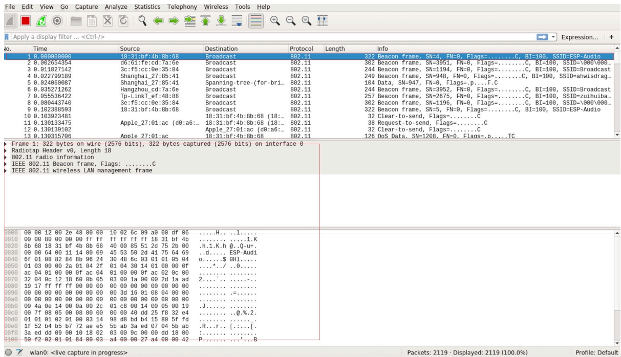
Fig. 46: Example of Packet List Details
