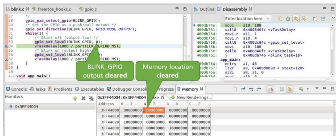
Fig. 26: Observing memory location 0x3FF44004 changing one bit to "OFF"
