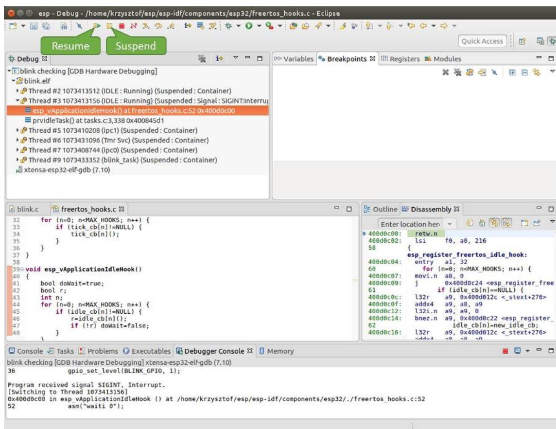
Fig. 22: Target halted manually
