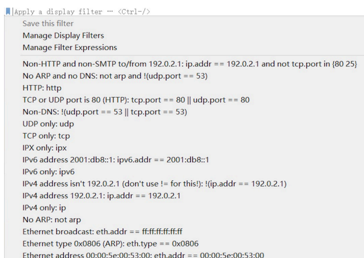
Fig. 42: Display Filter Dialogue Box
