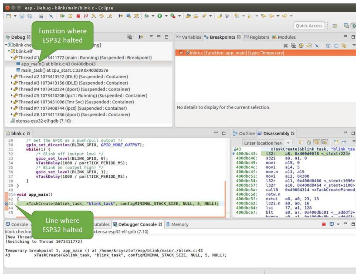
Fig. 18: Target halted during debugging
