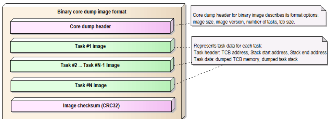
Fig. 6: Core Dump Binary Image Format
