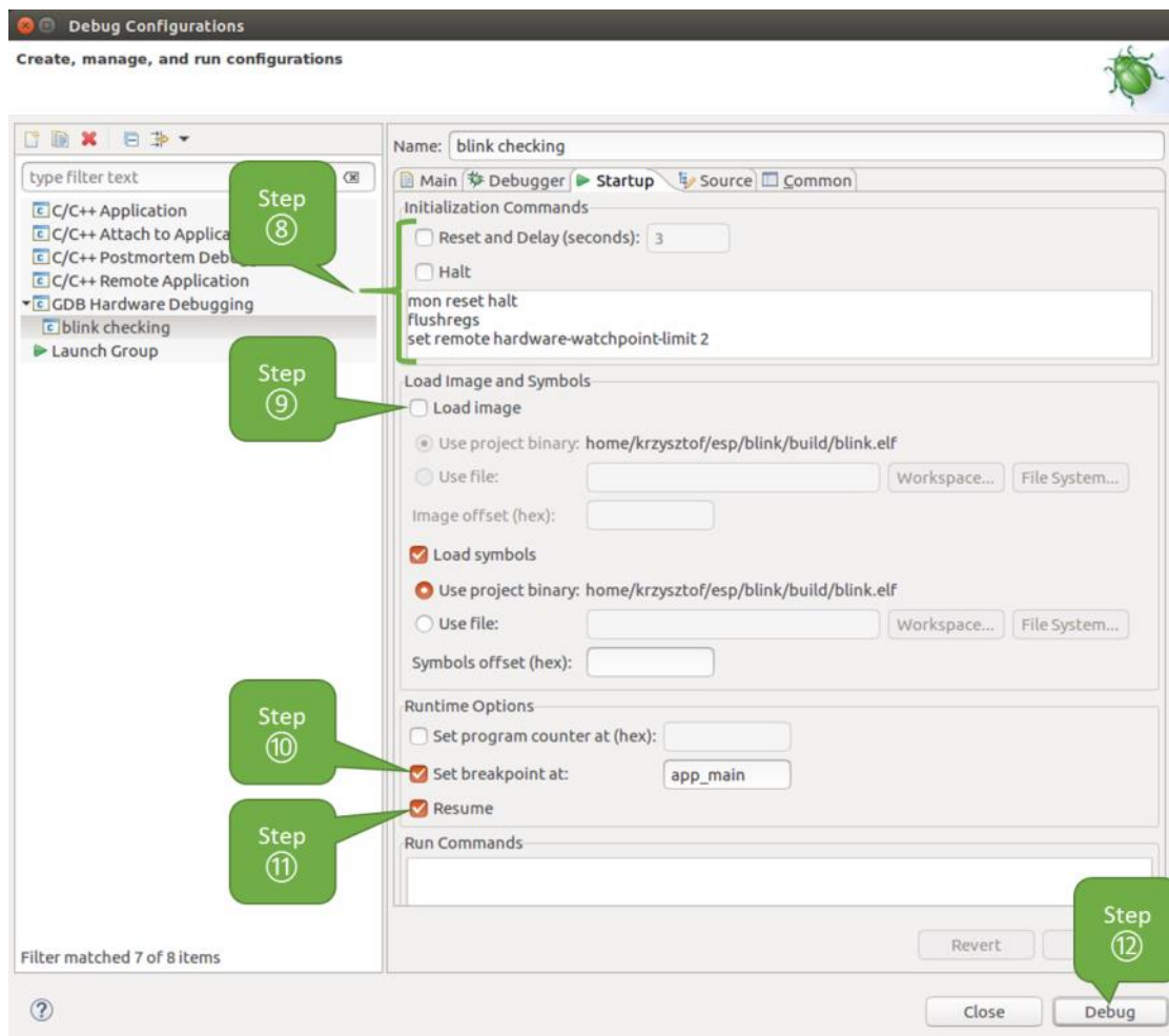
Fig. 15: Configuration of GDB Hardware Debugging - Startup tab
