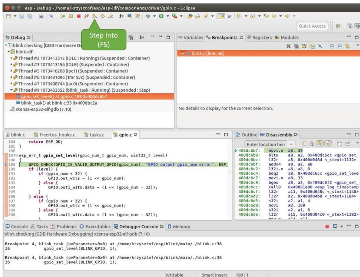
Fig. 24: Stepping through the code with "Step Into (F5)"
