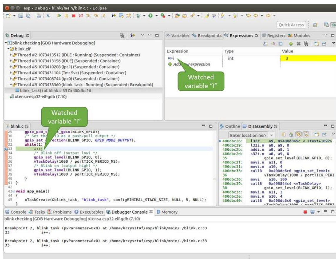
Fig. 27: Watching program variable "i"
