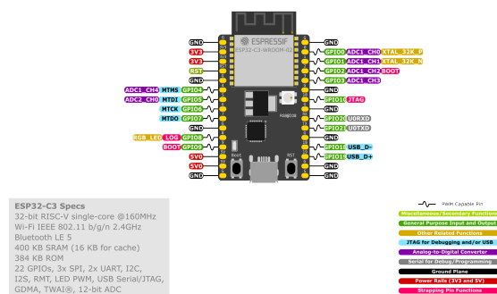
Fig. 8: ESP32-C3-DevKitC-02 Pin Layout (click to enlarge)
