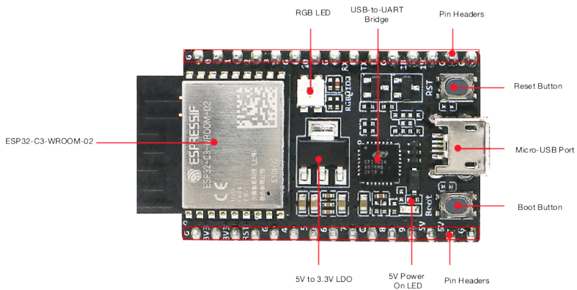
Fig. 6: ESP32-C3-DevKitC-02 - front
