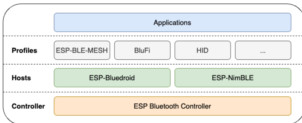
Fig. 3: ESP32-C3 Bluetooth Stack Architecture
