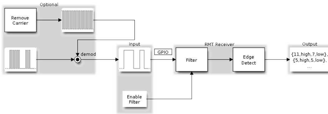
Fig. 20: RMT Receiver Overview
