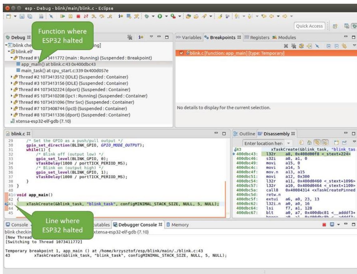
Fig. 31: Target halted during debugging
