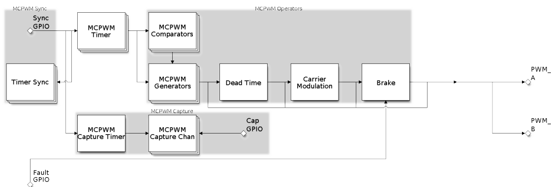
Fig. 15: MCPWM Overview
