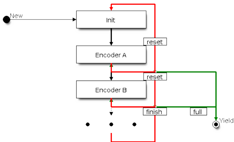
Fig. 22: RMT Encoder Chain
