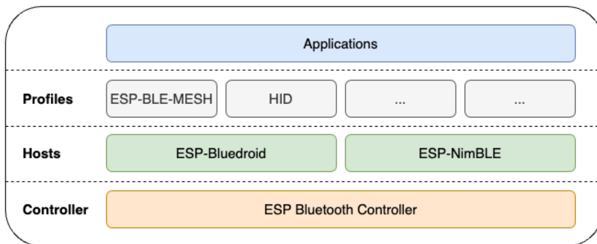
Fig. 2: ESP32-H2 Bluetooth Stack Architecture
