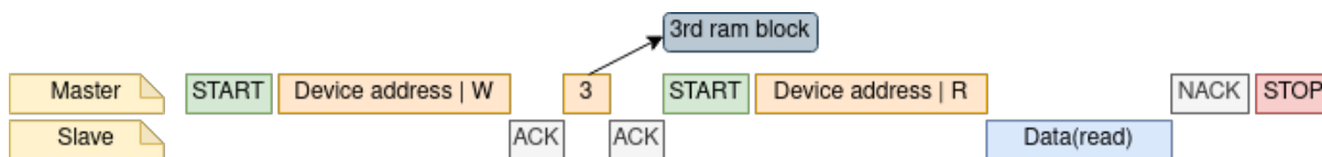
Fig. 11: Get data from I2C slave RAM
