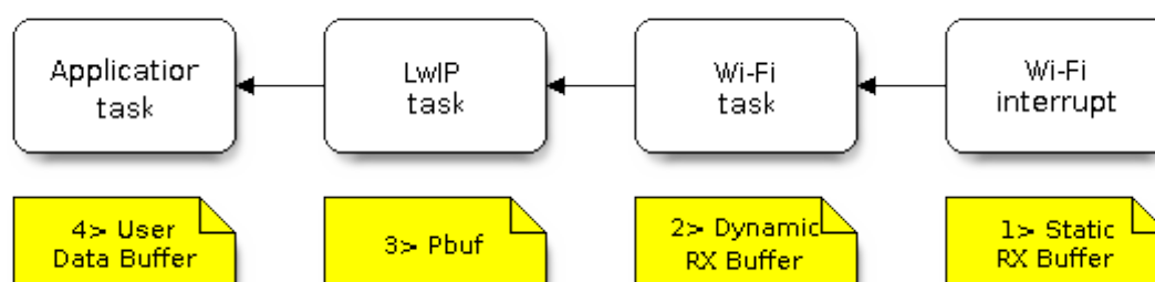
Fig. 41: RX Buffer Allocation
