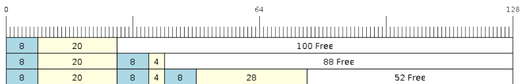
Fig. 36: Sending items to No-Split or Allow-Split ring buffers
