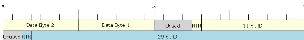
Fig. 29: Bit layout of single filter mode (Right side MSBit)
