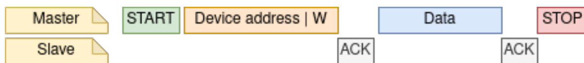
Fig. 6: I2C master write to slave
