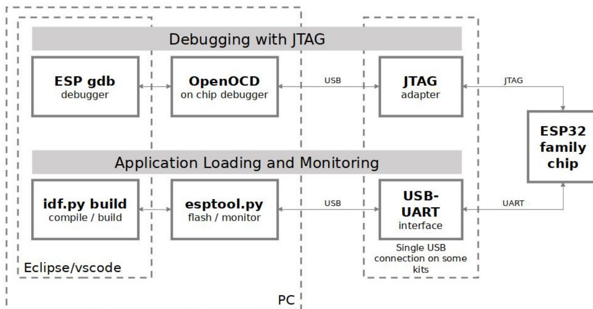
Fig. 45: JTAG debugging - overview diagram
