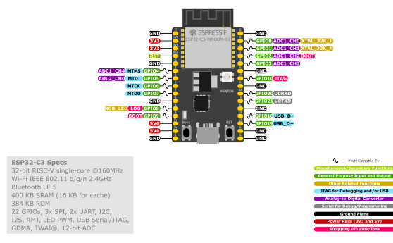
Fig. 8: ESP32-C3-DevKitC-02 Pin Layout (click to enlarge)
