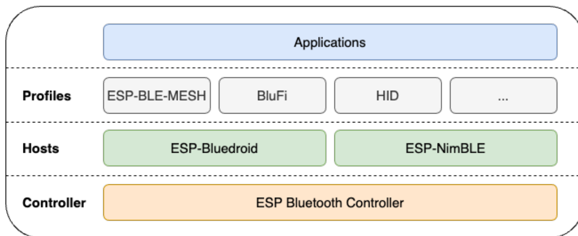
Fig. 3: ESP32-C6 Bluetooth Stack Architecture
