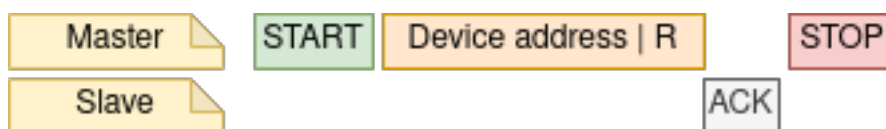
Fig. 11: I2C master probe
