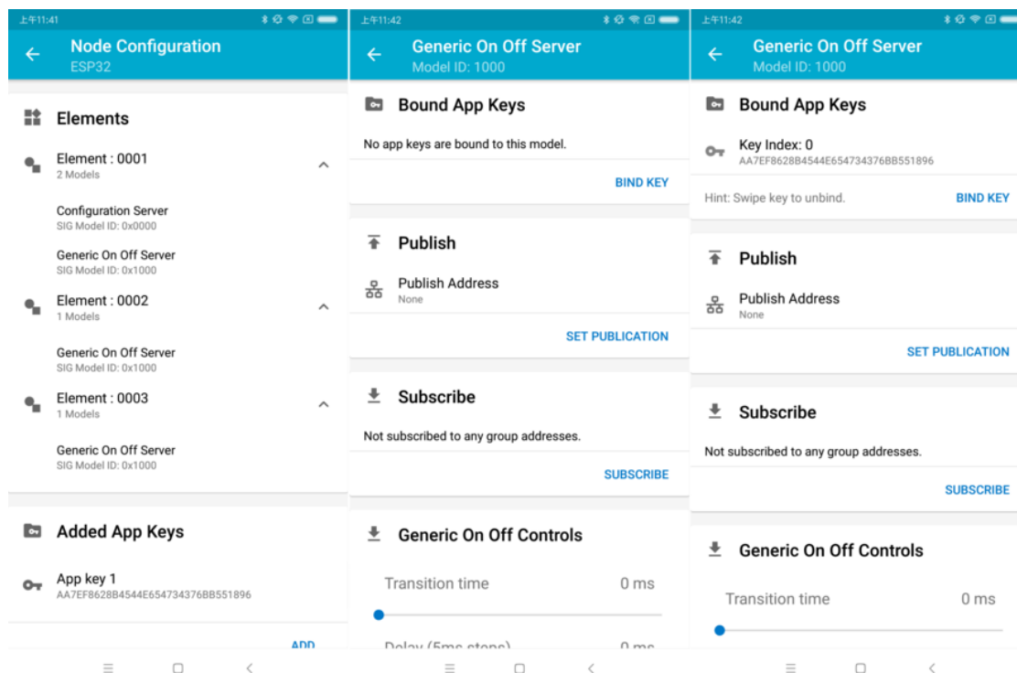
Fig. 17: nRF Mesh - Model Bind AppKey
