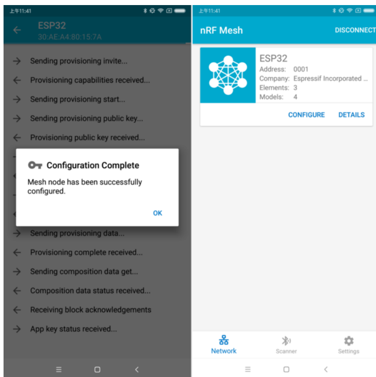
Fig. 13: nRF Mesh - Configuration Complete
