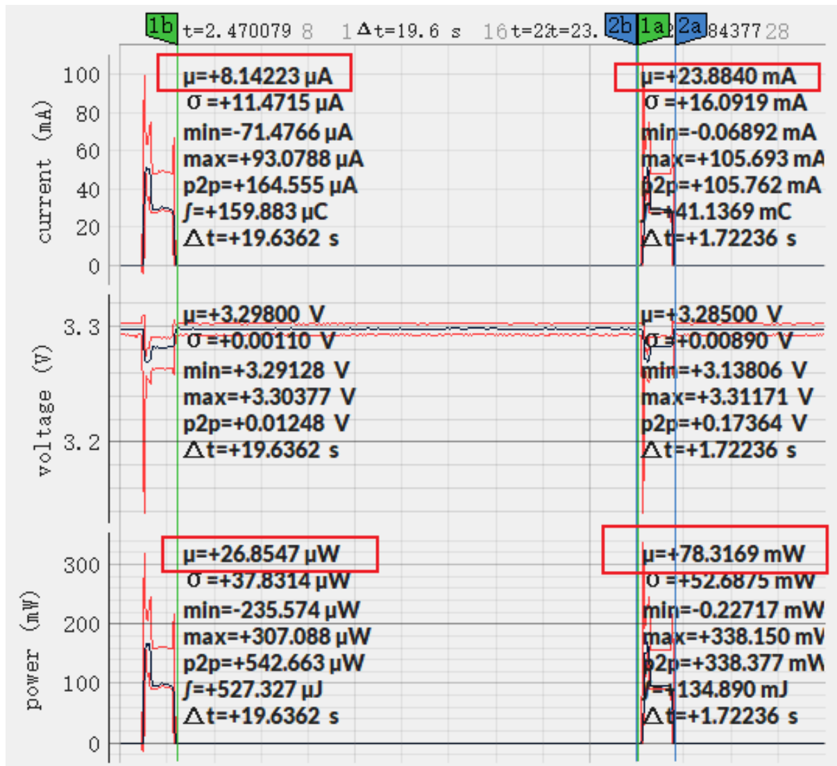
Fig. 8: Current Waveform of ESP32-S3-WROOM-1 (click to enlarge)
