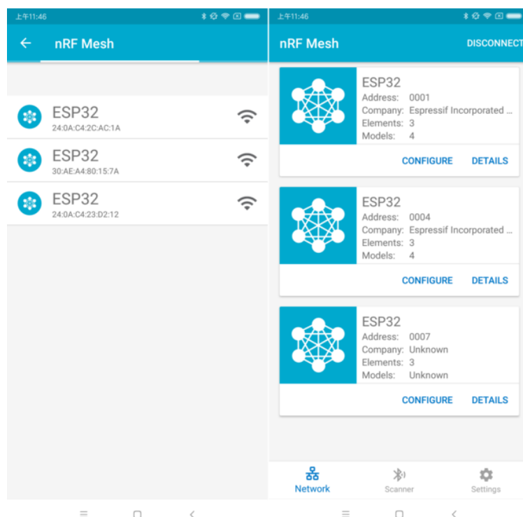
Fig. 16: nRF Mesh - Reconnect - Three Nodes
