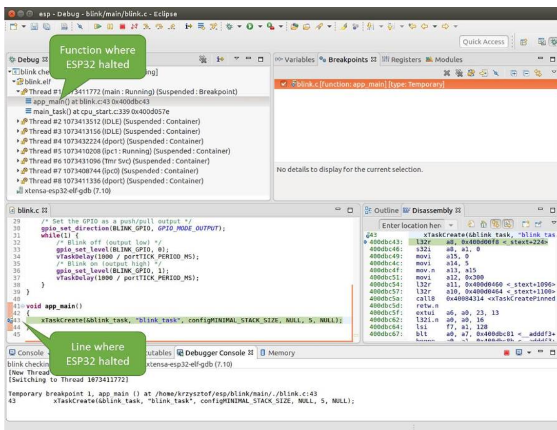
Fig. 29: Target halted during debugging
