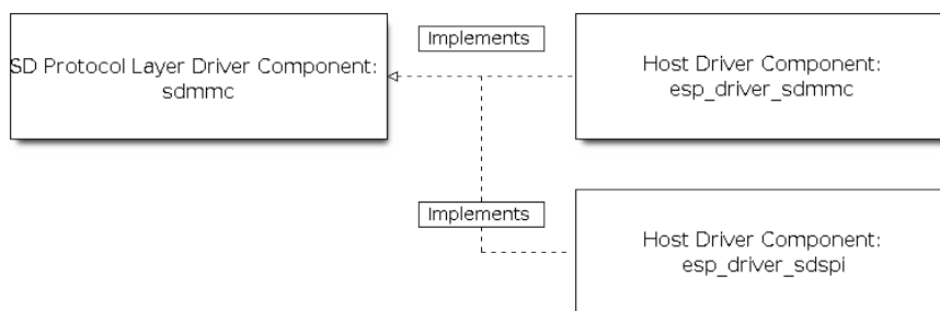
Fig. 32: SD Host Side Component Architecture
