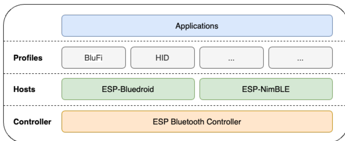
Fig. 3: ESP32-C2 Bluetooth Stack Architecture
