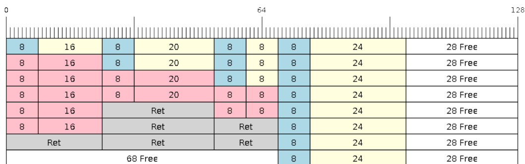
Fig. 21: Retrieving/Returning items in No-Split and Allow-Split ring buffers
