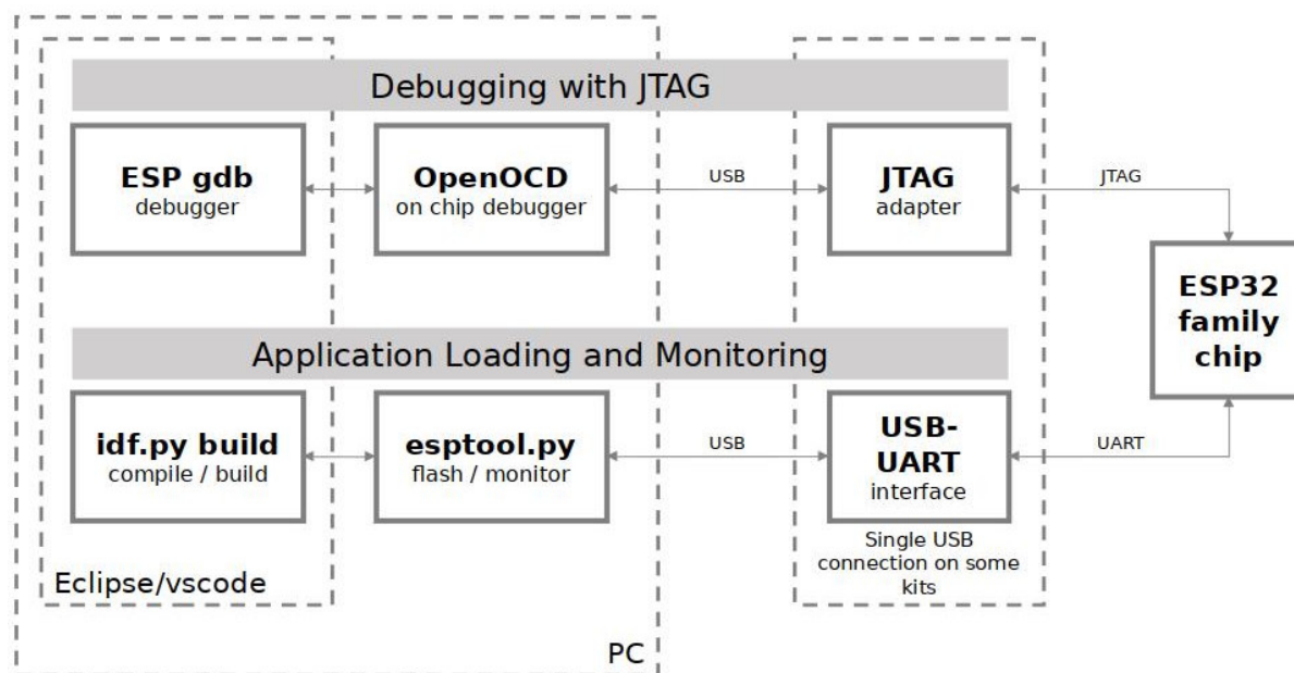
Fig. 14: JTAG debugging - overview diagram
