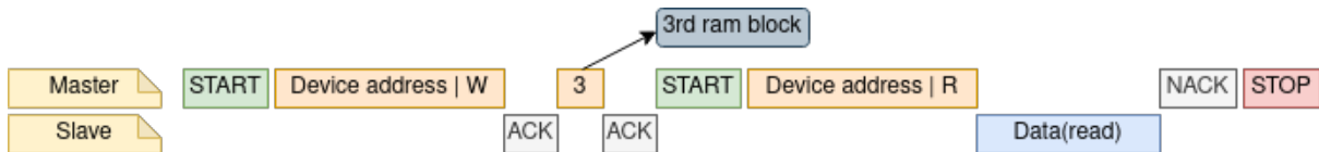
Fig. 11: Get data from I2C slave RAM
