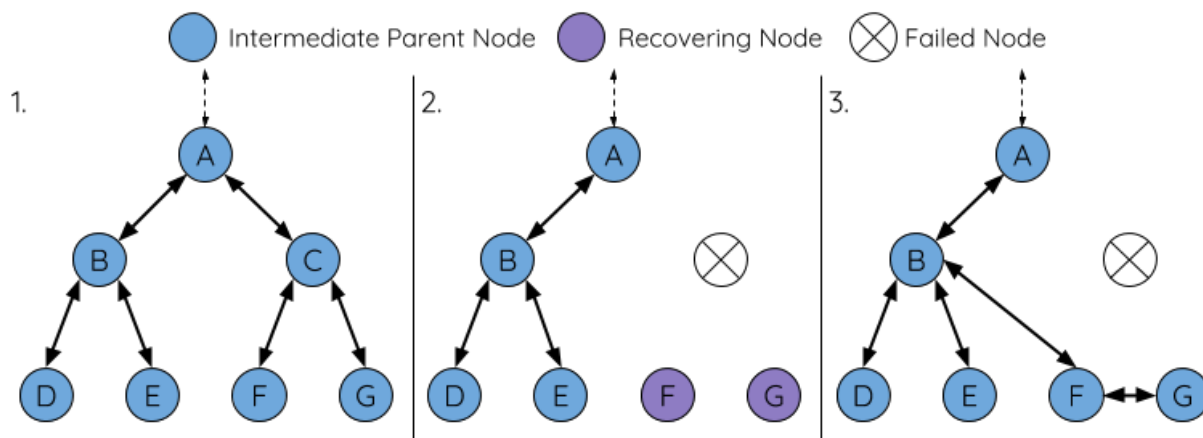
Fig. 58: Self Healing From Intermediate Parent Node Failure
