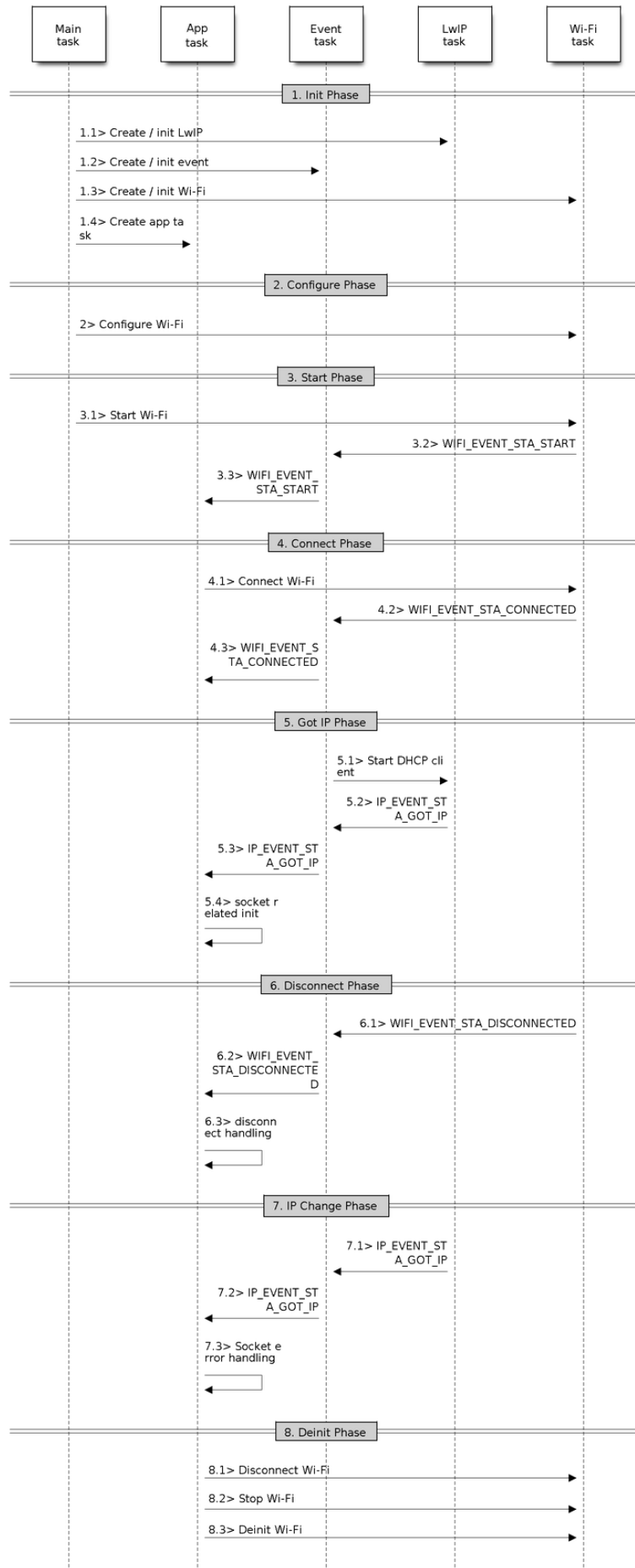
Fig. 83: Sample Wi-Fi Event Scenarios in Station Mode
