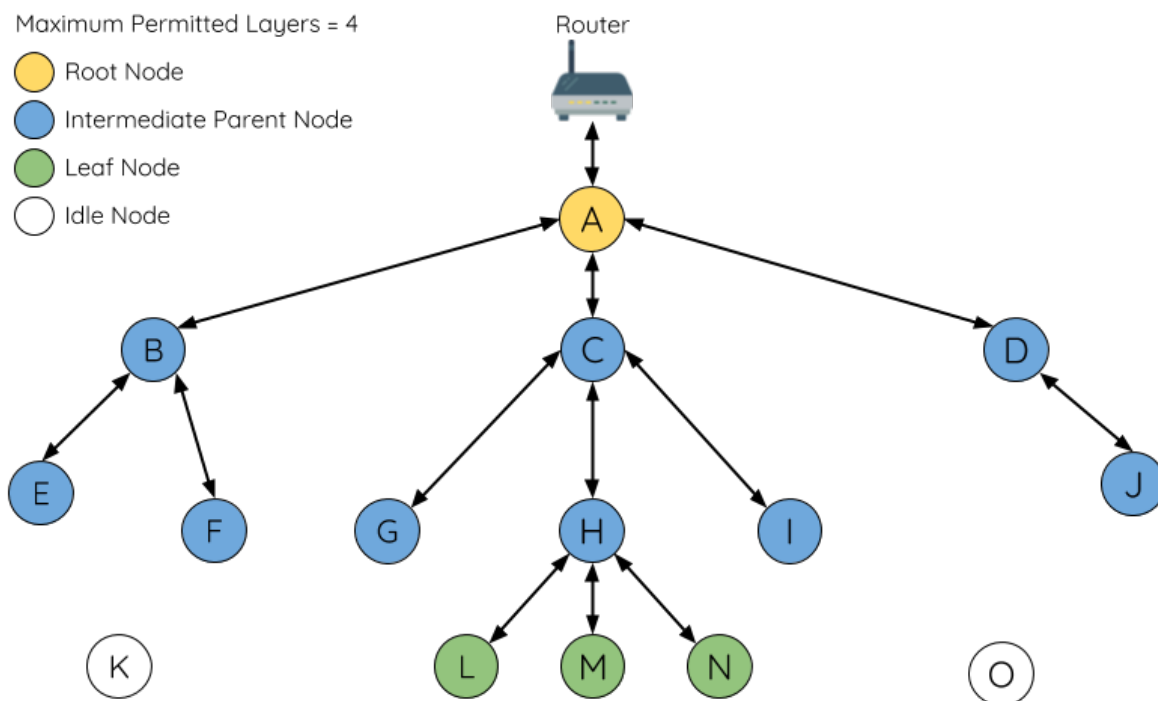
Fig. 49: ESP-WIFI-MESH Node Types
