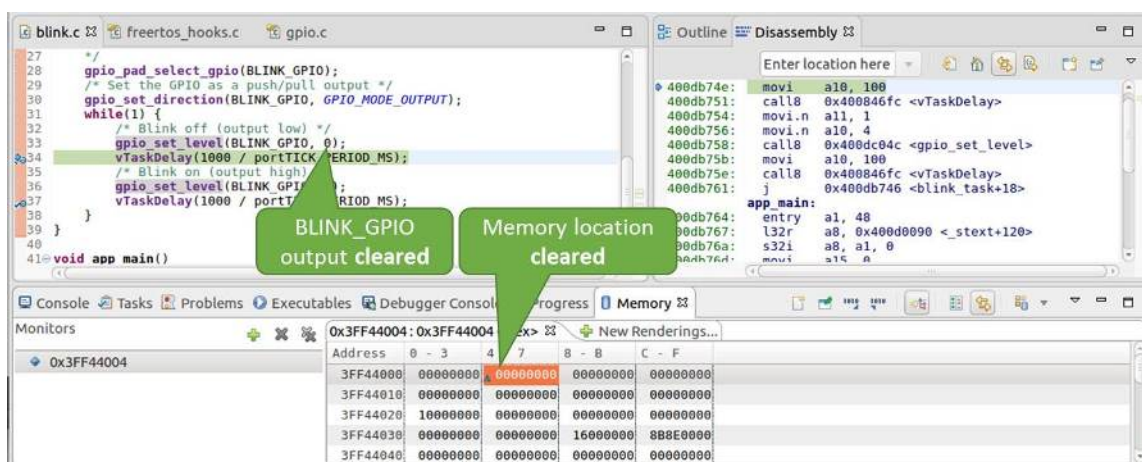
Fig. 78: Observing memory location 0x3FF44004 changing one bit to "OFF"
