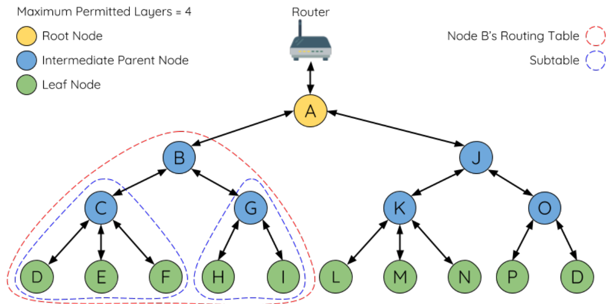
Fig. 52: ESP-WIFI-MESH Routing Tables Example
