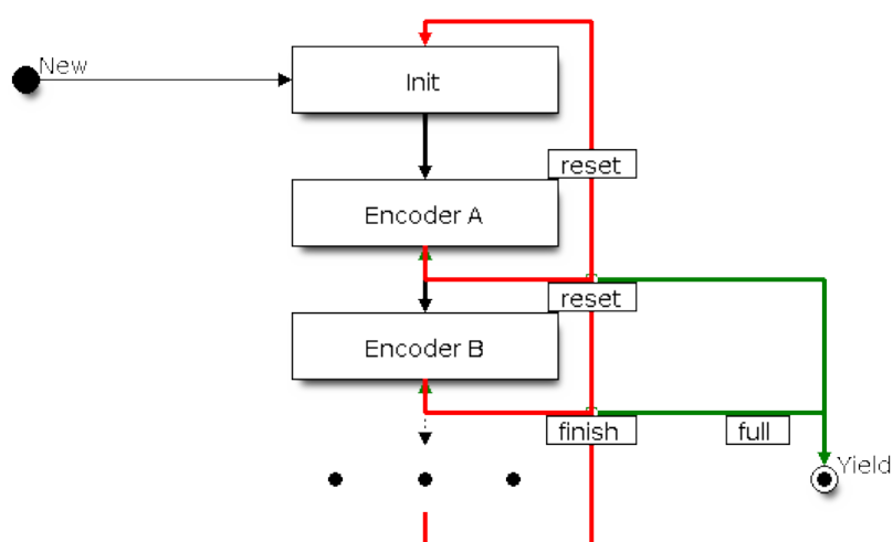
Fig. 24: RMT Encoder Chain
