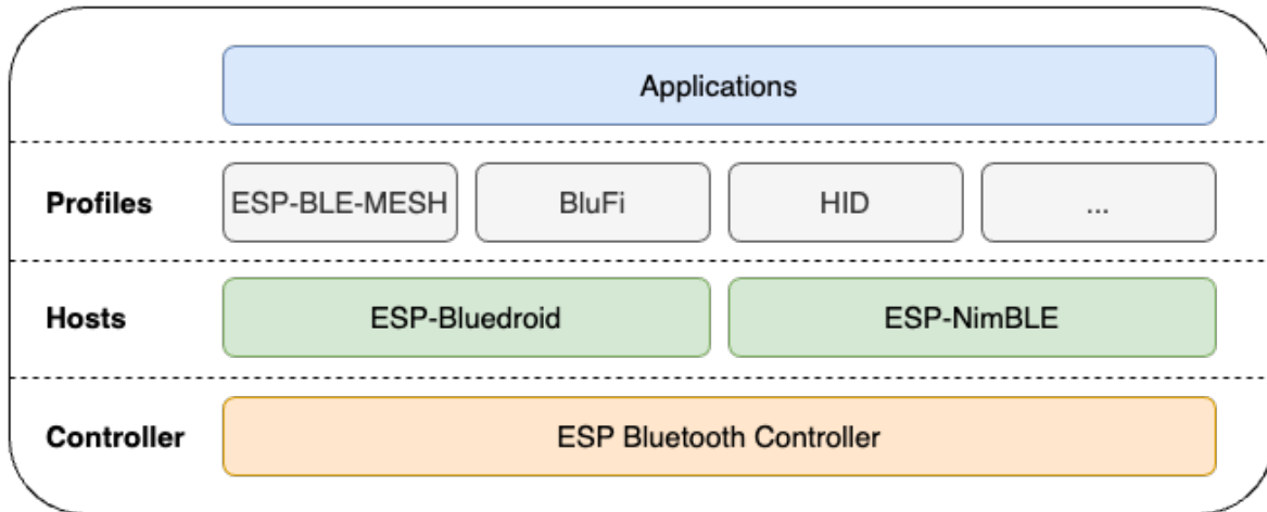
Fig. 2: ESP32-C3 Bluetooth LE Stack Architecture
