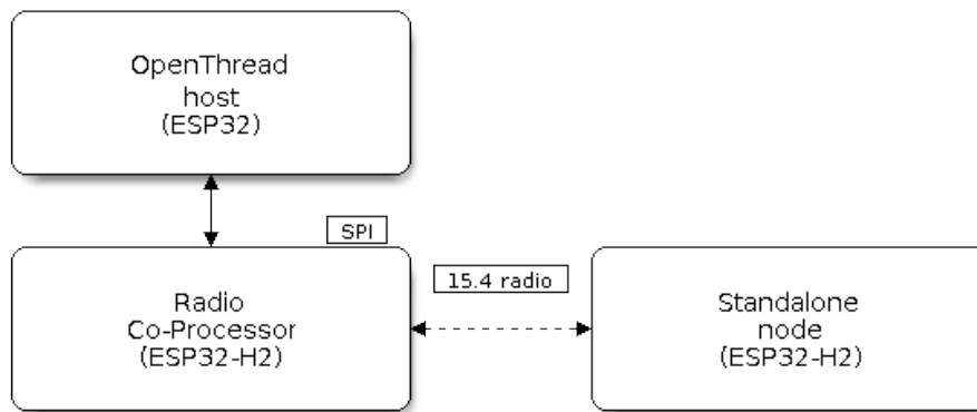
Fig. 79: OpenThread device modes
