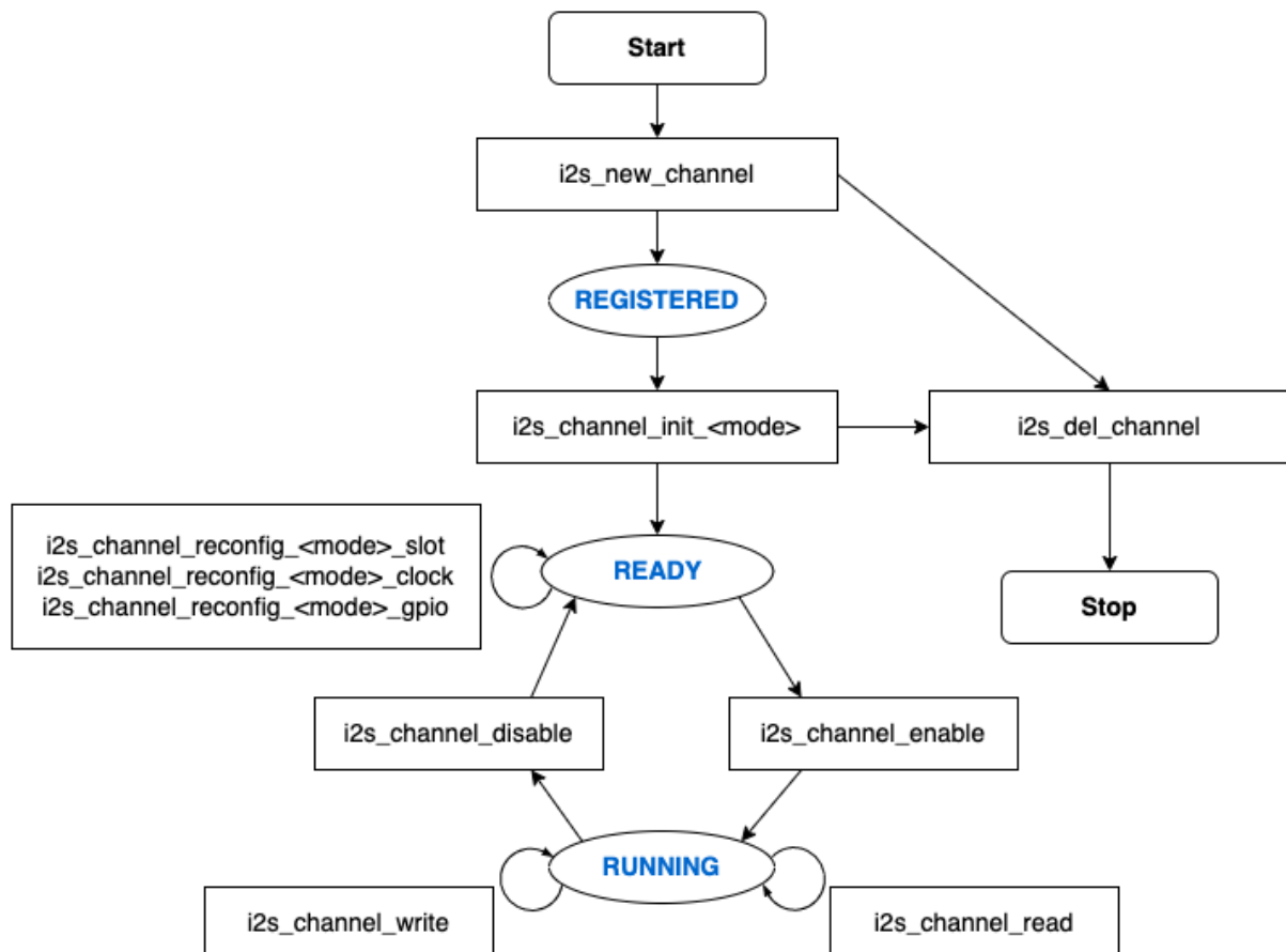
Fig. 14: I2S Finite State Machine
