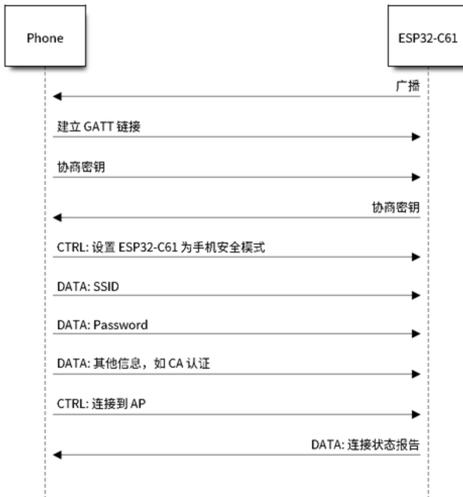
图 22: BluFi Flow Chart
