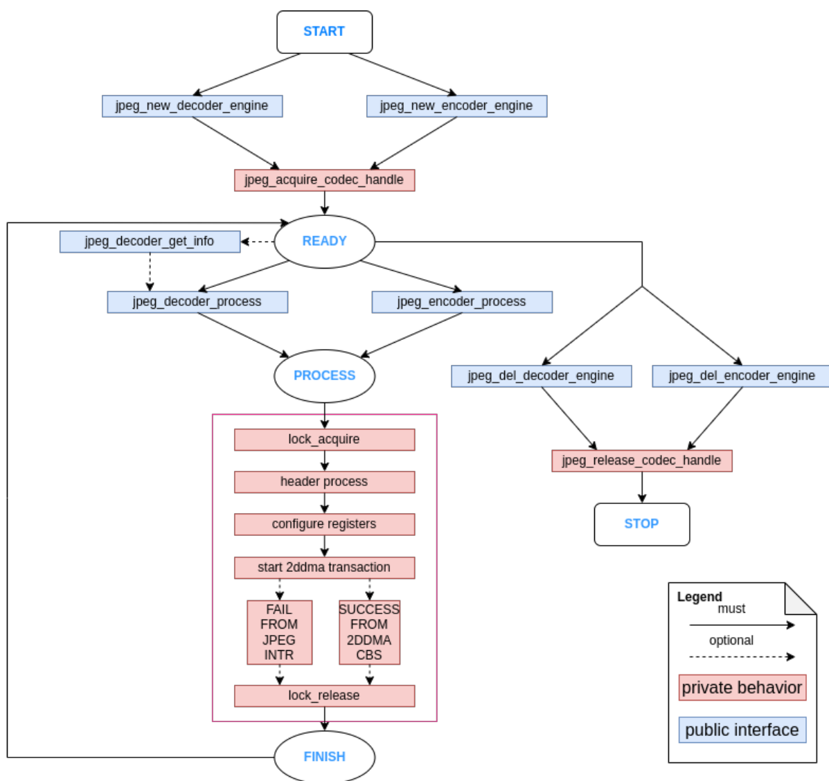
图 24: JPEG finite state machine
