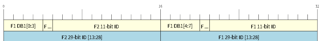
图 36: Bit layout of dual filter mode (Right side MSBit)
