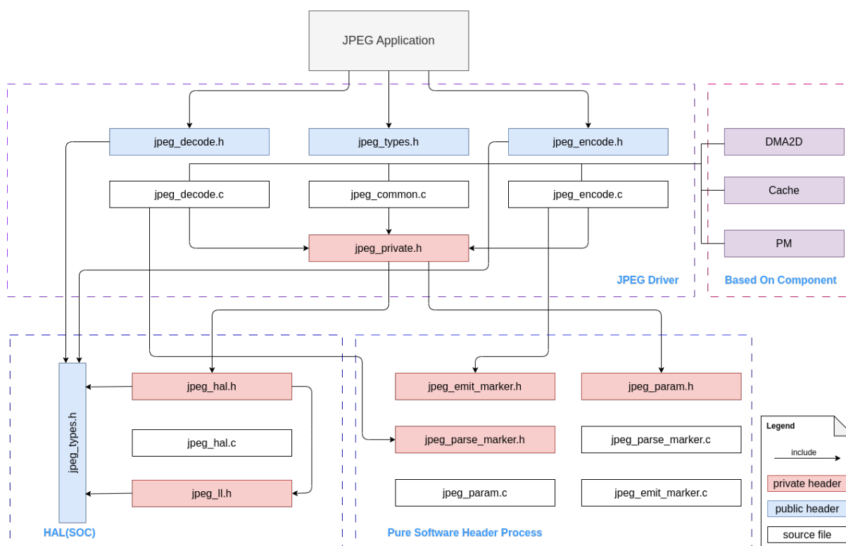
图 32: JPEG driver file structure
