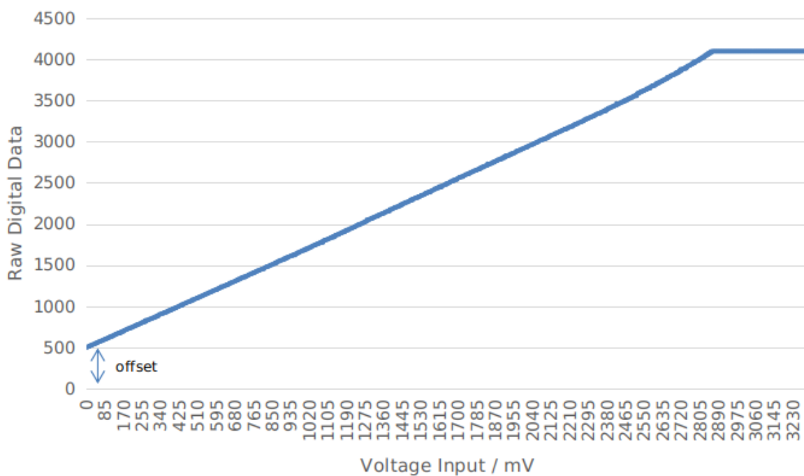
ADC Characteristics Before Calibration
