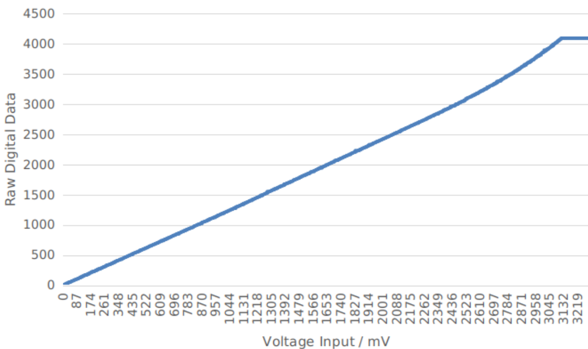
ADC Characteristics After HW Calibration
