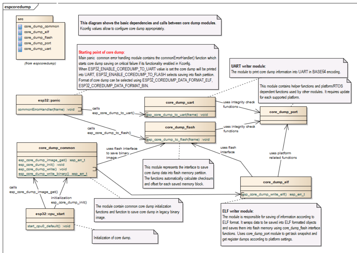
图 20: Core dump implementation overview
