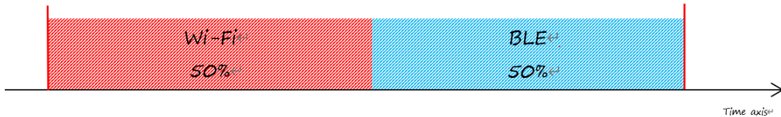
图 77: Wi-Fi CONNECTED 和 BLE CONNECTED 共存状态下时间片划分图
