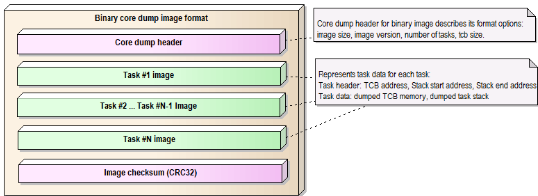
图 19: Core dump binary image format
