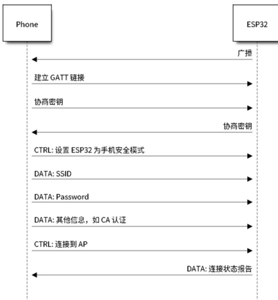
图 36: BluFi Flow Chart
