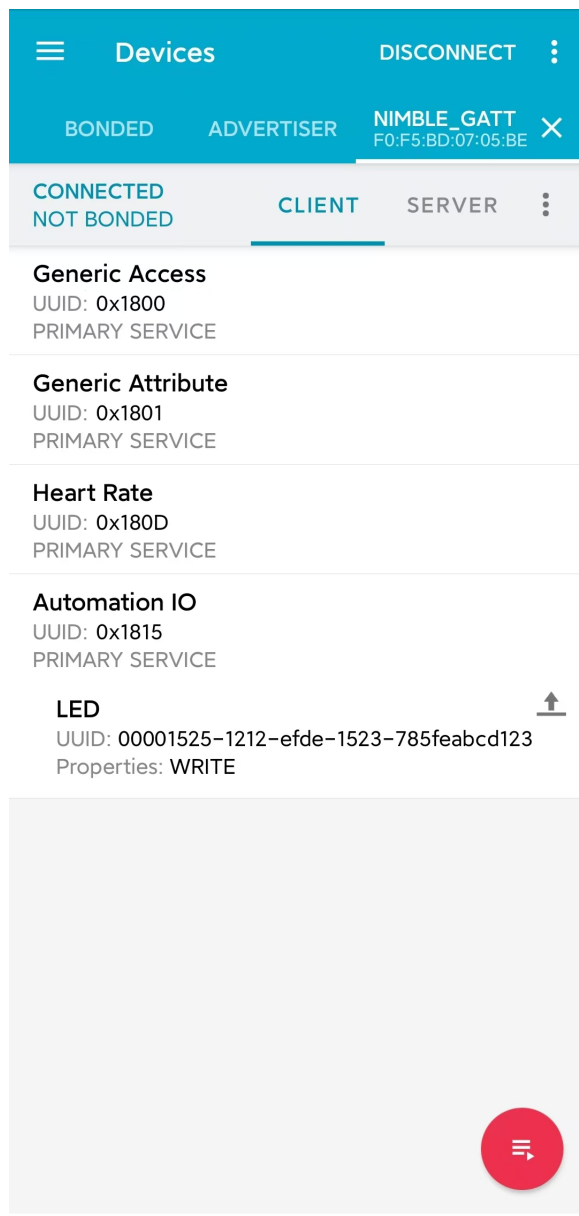
图 10: Automation IO Service
