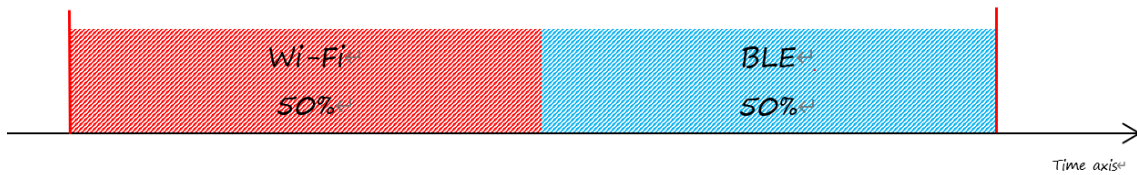
图 97: Wi-Fi CONNECTED 和 BLE CONNECTED 共存状态下时间片划分图
