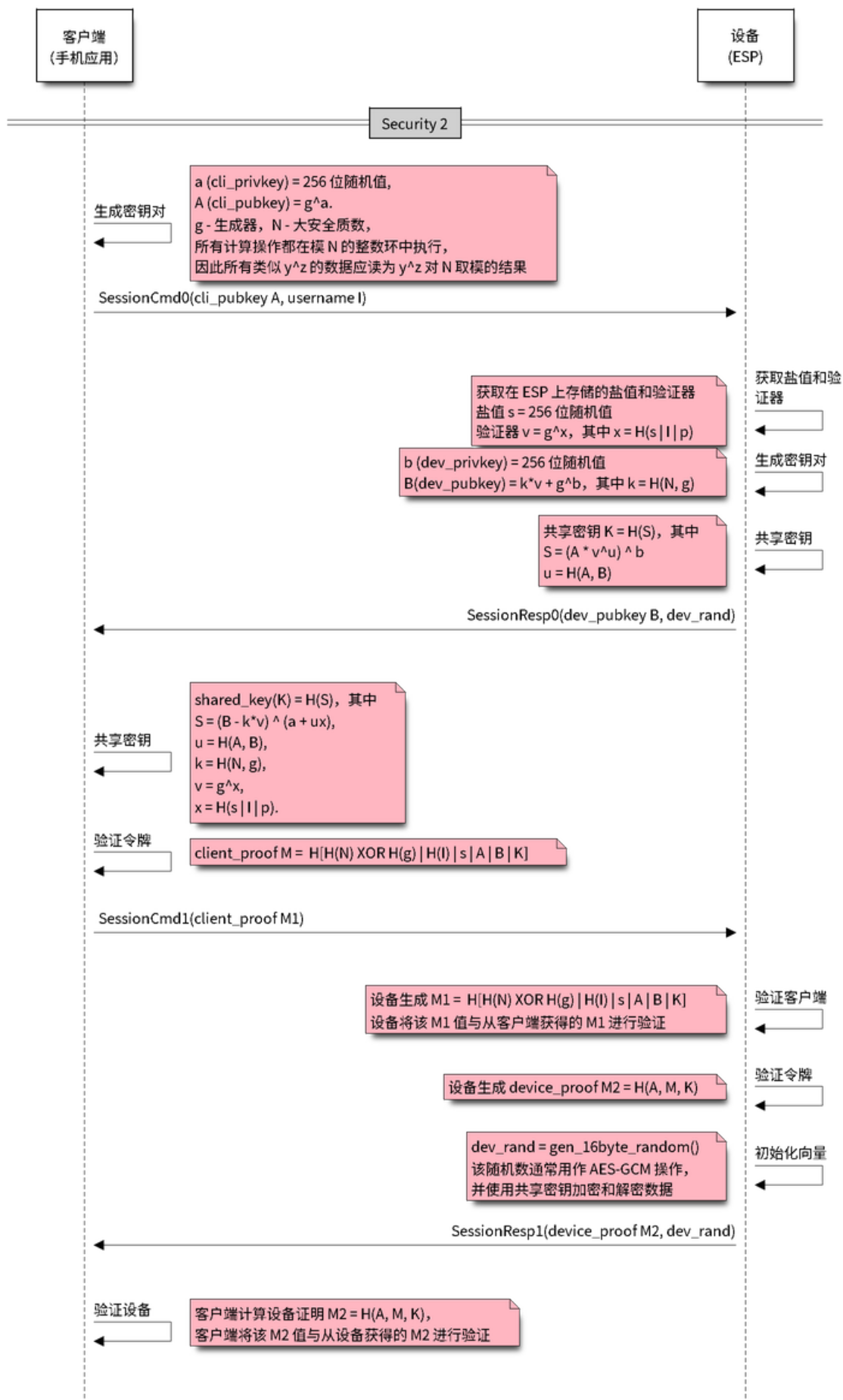
图 9: Security 2
