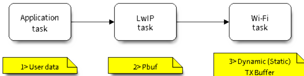
图 34: TX Buffer Allocation
