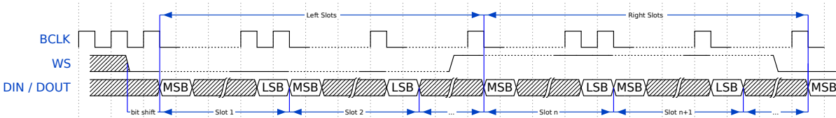
TDM Philips Timing Diagram
