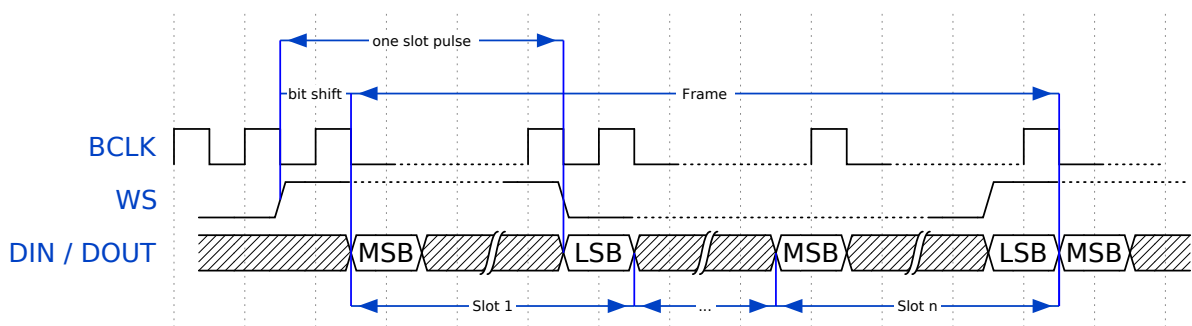
TDM PCM (long) Timing Diagram
