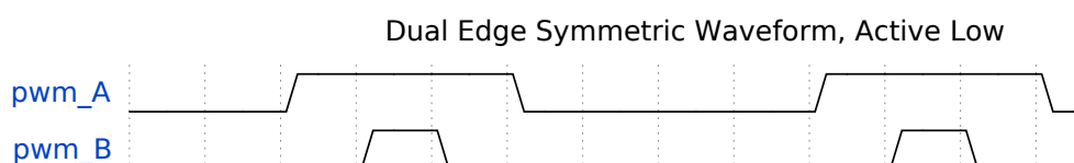
Symmetric Dual Edge Active Low
