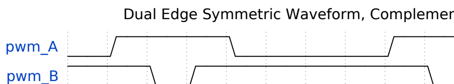
Symmetric Dual Edge Complementary
