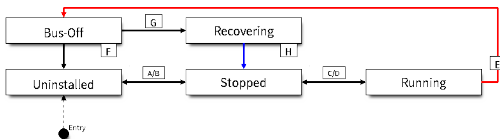
图 28: State transition diagram of the TWAI driver (see table below)
