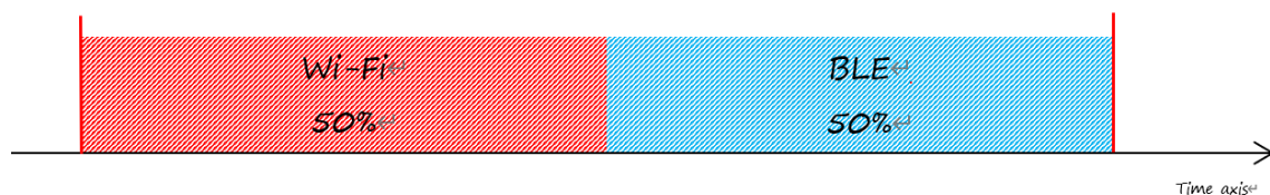
图 39: Wi-Fi CONNECTED 和 BLE CONNECTED 共存状态下时间片划分图
