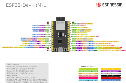
图 8: ESP32-DevKitM-1 (点击放大)
