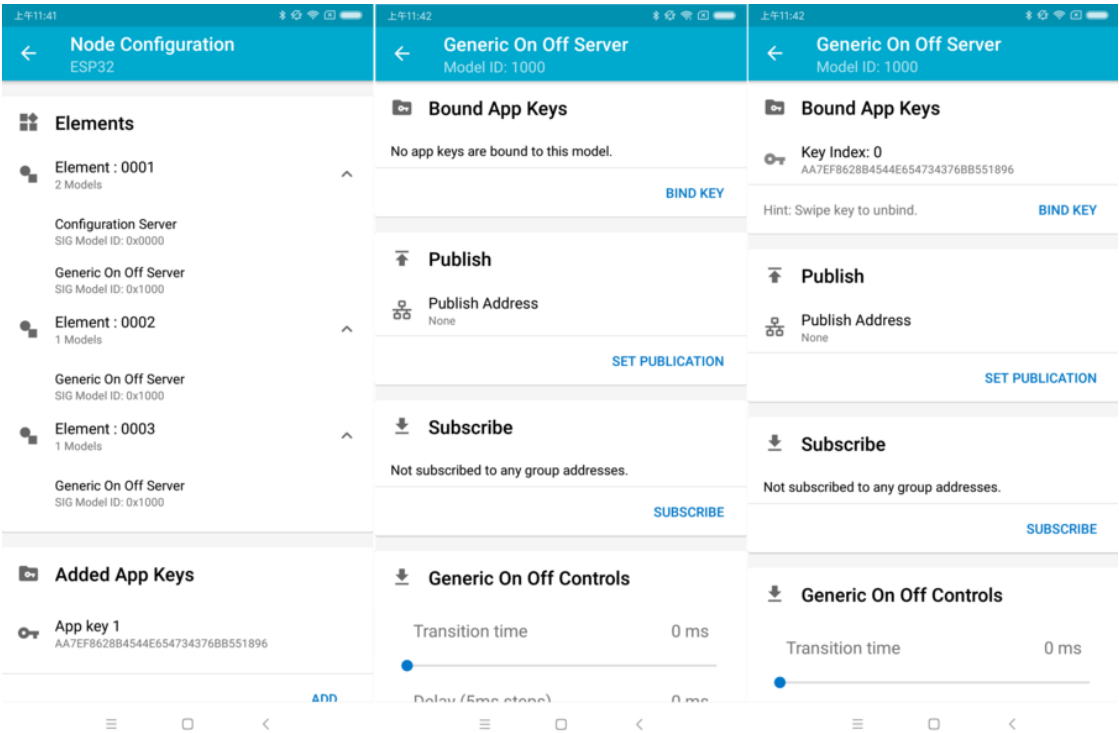
图 31: nRF Mesh - Model Bind AppKey
