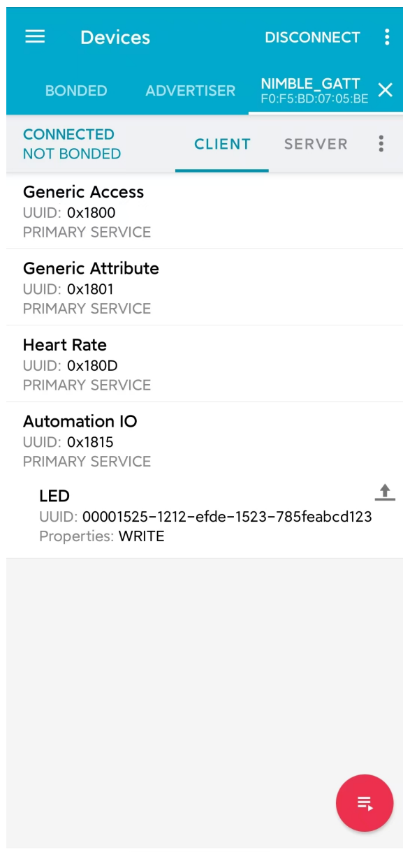
图 10: Automation IO Service
