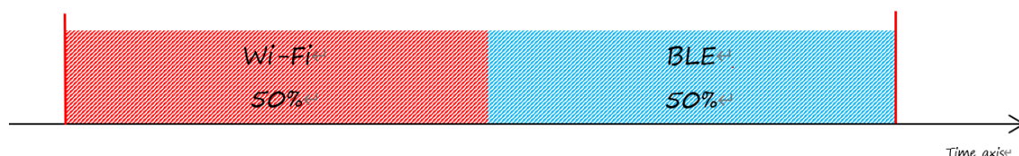
图 39: Wi-Fi CONNECTED 和 BLE CONNECTED 共存状态下时间片划分图
