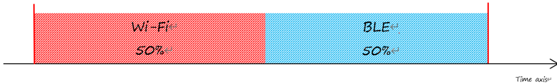
图 18: Wi-Fi CONNECTED 和 BLE CONNECTED 共存状态下时间片划分图
