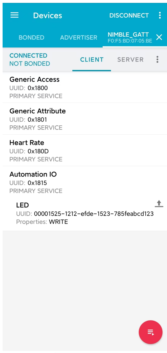
图 9: Automation IO Service
